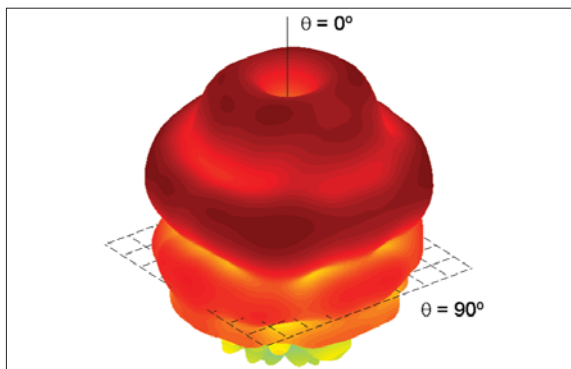
■ Figure 4. (a) Magnetic monopole antenna. (b) 2D antenna gain pattern and (c) 3D antenna gain pattern, both expressed in dB. 2D and 3D gain patterns have been measured with the antenna mounted over a finite metallic plane with 1 m by 1 m dimensions.
