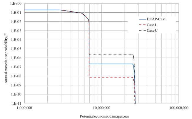
Fig. 14. FD-curves for the DEAP-Case and sensitivity analysis.
