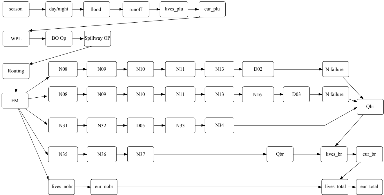
Fig. 8. Risk Model 2. Pluvial flooding and river flooding including the existence of the dam.
