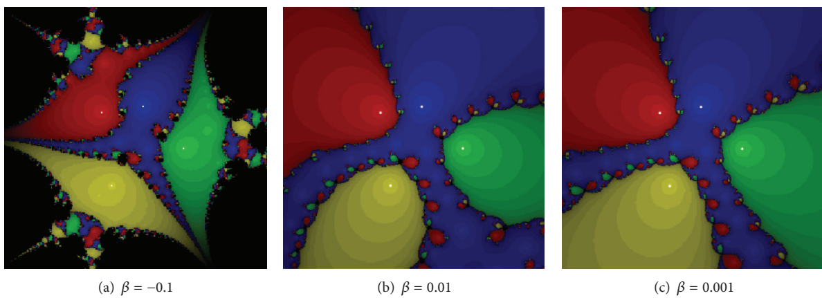
FIGURE 8: Scheme (3) for the test problem 4.
