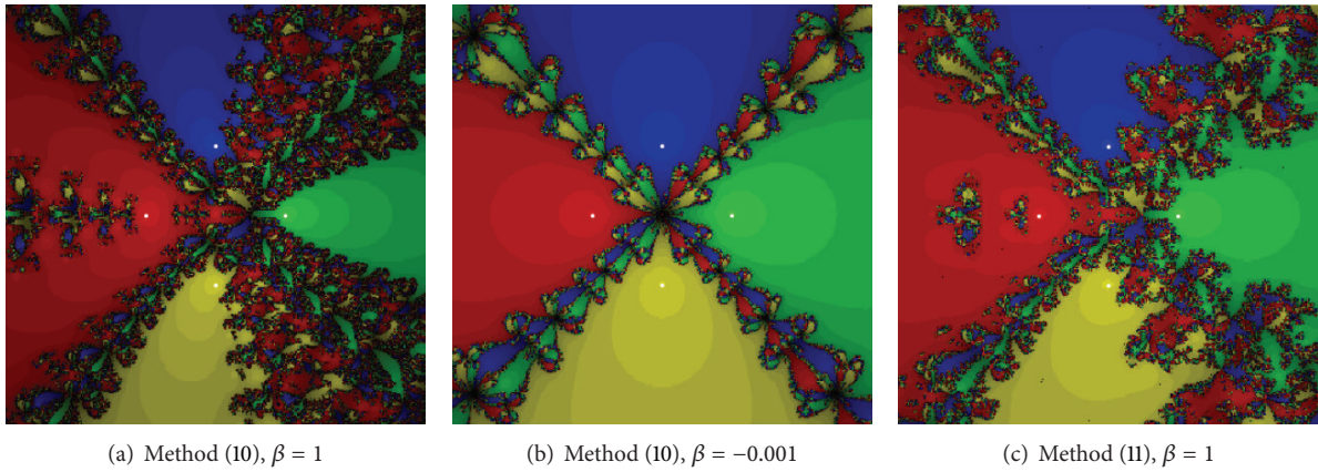
FIGURE 16: Basins of attraction for the test problem 1.
