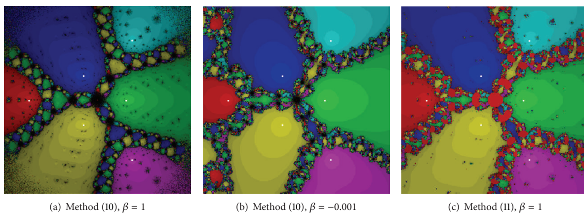
FIGURE 19: Basins of attraction for the test problem 2.
