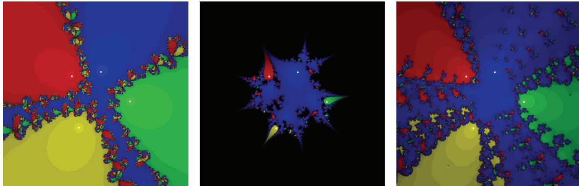
(a) Method (11), \beta = -0.001
