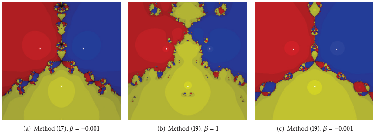
FIGURE 27: Basins of attraction for the test problem 5.
