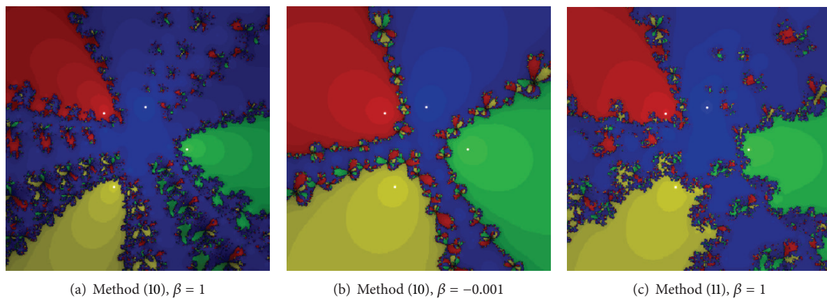
FIGURE 22: Basins of attraction for the test problem 4.
