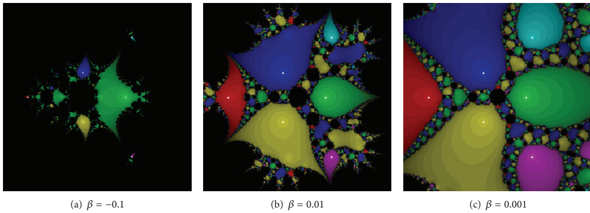
FIGURE 4: Scheme (3) for the test problem 2.
