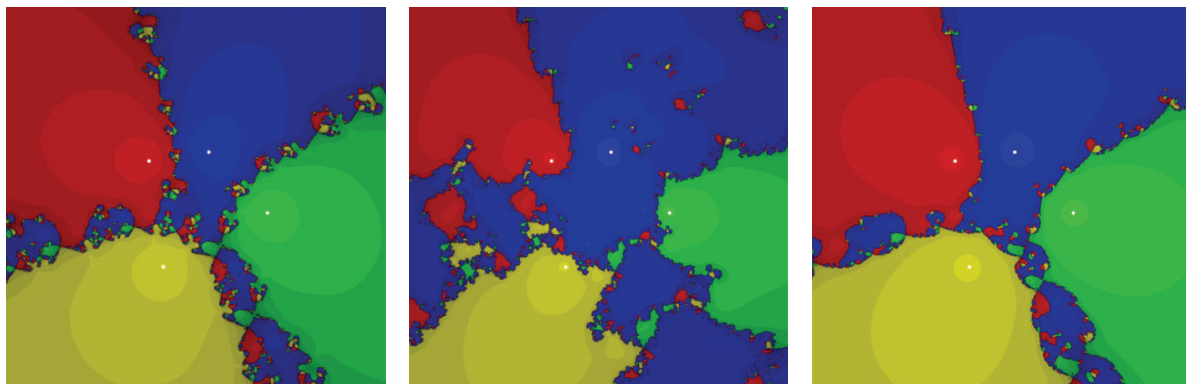
(a) Method (17), \beta = -0.001
