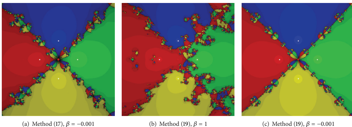
FIGURE 18: Basins of attraction for the test problem 1.
