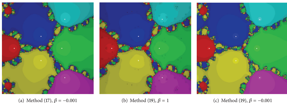
FIGURE 21: Basins of attraction for the test problem 2.
