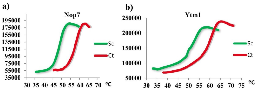
Figure 4.20 Proteins from C. thermophilum are more thermostable.
