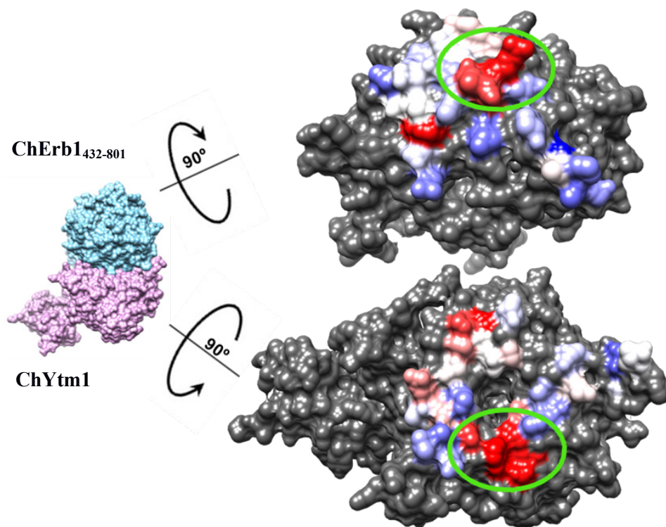
Figure 4.41. Conservation of the surface involved in ChErb1 432-801 -ChYtm1 interaction. The colored surfaces of ChErb1Ct (top) and ChYtm1 (bottom) show the area that mediates the binding between both molecules. The most variable residues are shown in blue and the most conserved one are depicted in red. Green circles mark the region that was chosen for mutant generation.
