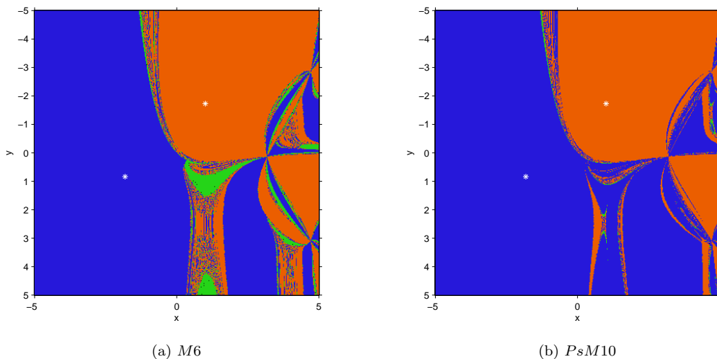
Figure 2: Real dynamical planes for system F_3(x) = 0 and methods M6 and PsM10
