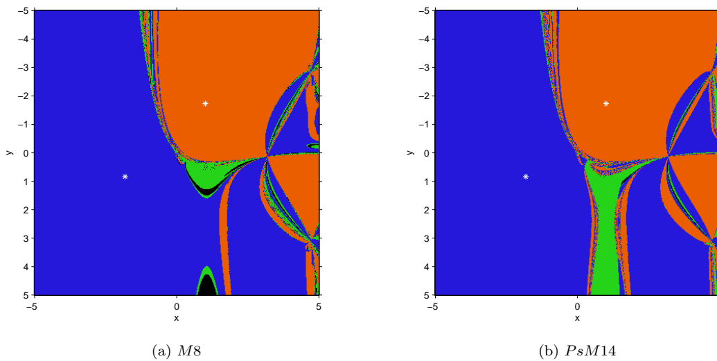
Figure 3: Real dynamical planes for system F_3(x) = 0 and methods M8 and PsM14
