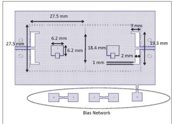
■ Figure 16. (Left): Photograph of the tunable filter during the 1-dB compression point measurement. (Right): Layout and dimensions of the fabricated tunable filter.
