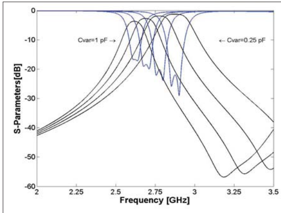
■ Figure 15. Simulation results of the fabricated filter for a varactor capacitance ranging from 0.25 pF ( f_0 = 2.88 GHz) to 1 pF ( f_0 = 2.64 GHz).
