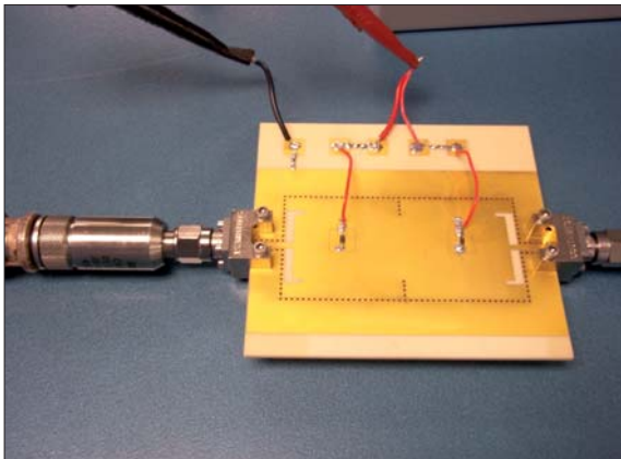
■ Figure 16. (Left): Photograph of the tunable filter during the 1-dB compression point measurement. (Right): Layout and dimensions of the fabricated tunable filter.
