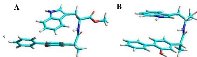
Figure 6. Geometry optimised (HyperChem Release 8.0.3 for Windows Molecular Model System, PM3) structure for ( S,S )- 1 (A) and ( S,R )- 1 (B).
