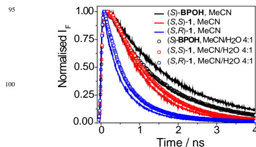
Figure 5. Kinetic decay traces ( \lambda_{exc} = 267 nm, \lambda_{em} = 330 nm, A_{267} = 0.2 ) for ( S )- BPOH (black), ( S,S )- 1 (red) and ( S,R )- 1 (blue) under air, in MeCN (solid line) and MeCN/H 2 O 4:1 (open circles).
