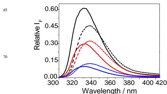
Figure 2. Fluorescence spectra of ( S )- BPOH (black), ( S,S )- 1 (red) and ( S,R )- 1 (blue) at λ exc = 267 nm, under air. Solid lines: MeCN; dashed lines: MeCN/H 2 O 4:1.
