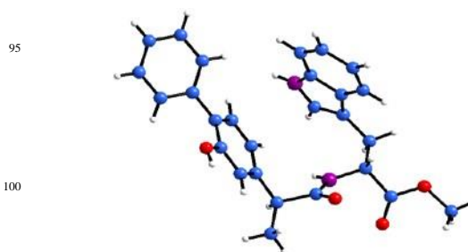
Figure 3. X-ray structure of compound ( S,R )- 1 .
