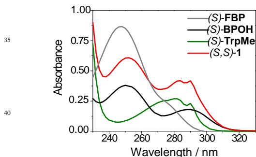
Figure 1. UV-Vis absorption spectra of ( S )- FBP (grey), ( S )- BPOH (black), ( S )- TrpMe (green) and ( S,S )- 1 (red) in acetonitrile at 5 × 10 -5 M concentration.
