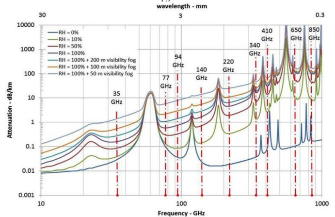
Fig. 1. Atmospheric attenuation curves under various levels of relative humidity (RH) and fog [3].
