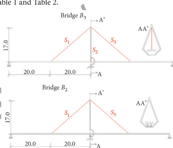
Fig. 2. Simplified examples of bridges B_2 and B_3 (dimensions in metres). Note: bridge B_2 has only 2 stays named S_1 and S_3 , and stay S_2 in bridge B_3 is aligned with the bridge mast
