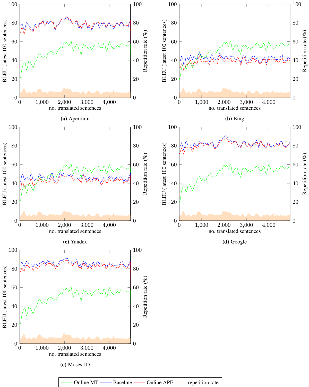
Figure A.15: Dynamics of online learning APE for the i3media corpus (Spanish to Catalan). The plots show the evolution of BLEU and repetition rate for a window of the latest 100 sentences, as the user completes the translation. The base system is compared to the APE system and a baseline online learning system.
