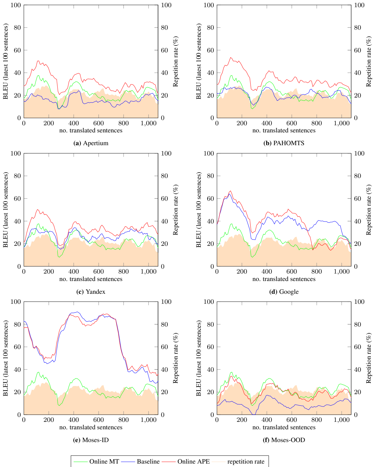
Figure A.13: Dynamics of online learning APE for the Xerox corpus (English to Spanish). The plots show the evolution of BLEU and repetition rate for a window of the latest 100 sentences, as the user completes the translation. The base system is compared to the APE system and a baseline online learning system.
