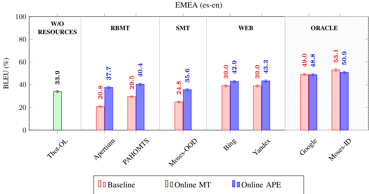
Figure 4: EMEA Spanish to English. Comparison between each MT system translations and their online post-editings. Online learning translation with Thot is considered as baseline system. Confidence intervals at 95%
