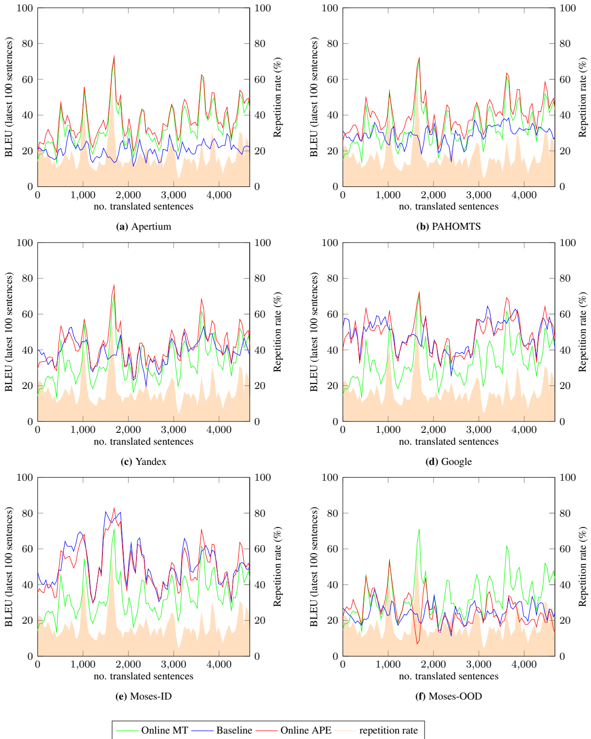
Figure A.12: Dynamics of online learning APE for the EMEA corpus (Spanish to English). The plots show the evolution of BLEU and repetition rate for a window of the latest 100 sentences, as the user completes the translation. The base system is compared to the APE system and a baseline online learning system.
