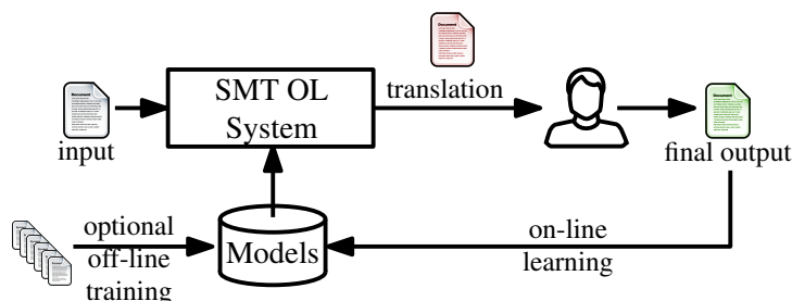
Figure 2: Diagram of an SMT system with OL.
