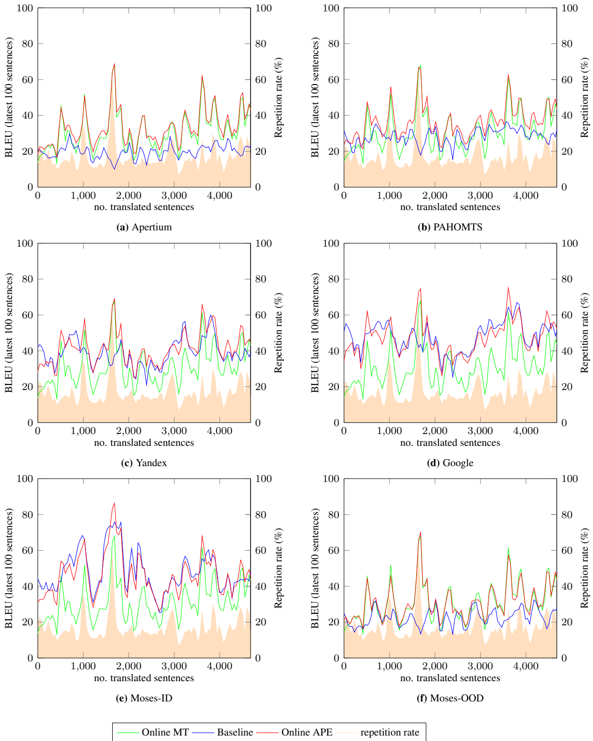
Figure A.11: Dynamics of online learning APE for the EMEA corpus (English to Spanish). The plots show the evolution of BLEU and repetition rate for a window of the latest 100 sentences, as the user completes the translation. The base system is compared to the APE system and a baseline online learning system.
