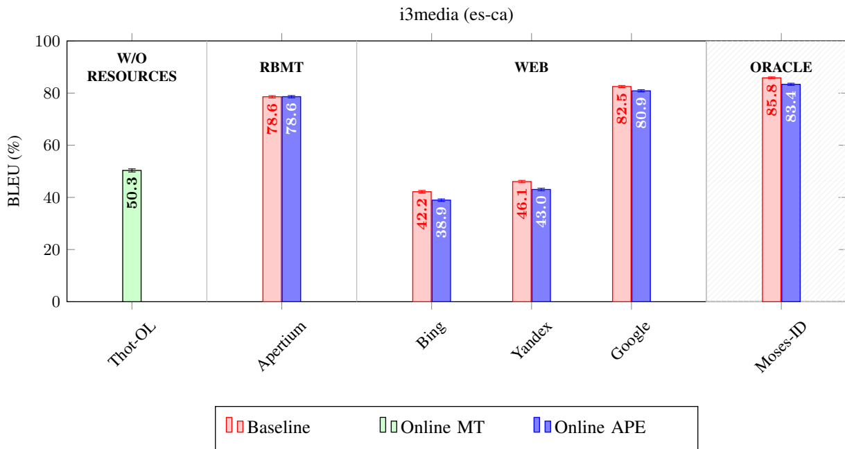
Figure 7: i3media Spanish to Catalan. Comparison between each MT system translations and their online post-editings. Online learning translation with Thot is considered as baseline system. Confidence intervals at 95%
