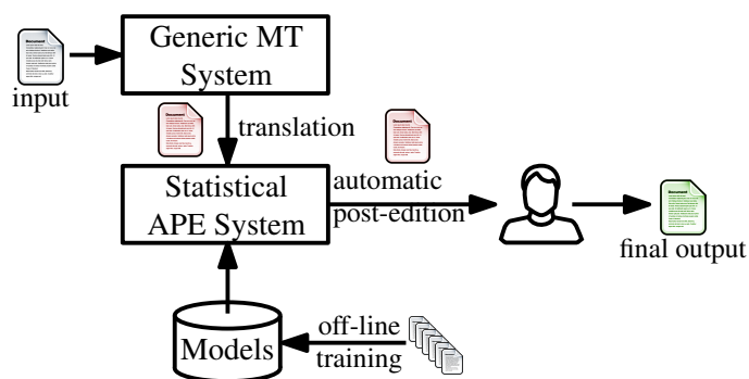
Figure 1: Diagram of an APE system.
