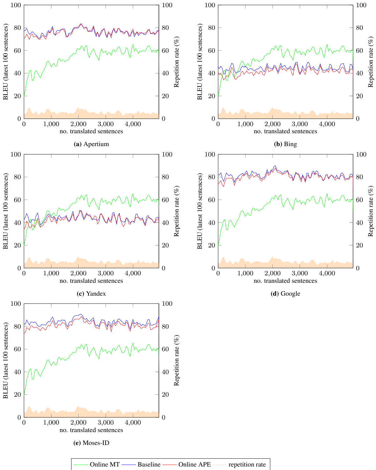
Figure A.16: Dynamics of online learning APE for the i3media corpus (Catalan to Spanish). The plots show the evolution of BLEU and repetition rate for a window of the latest 100 sentences, as the user completes the translation. The base system is compared to the APE system and a baseline online learning system.
