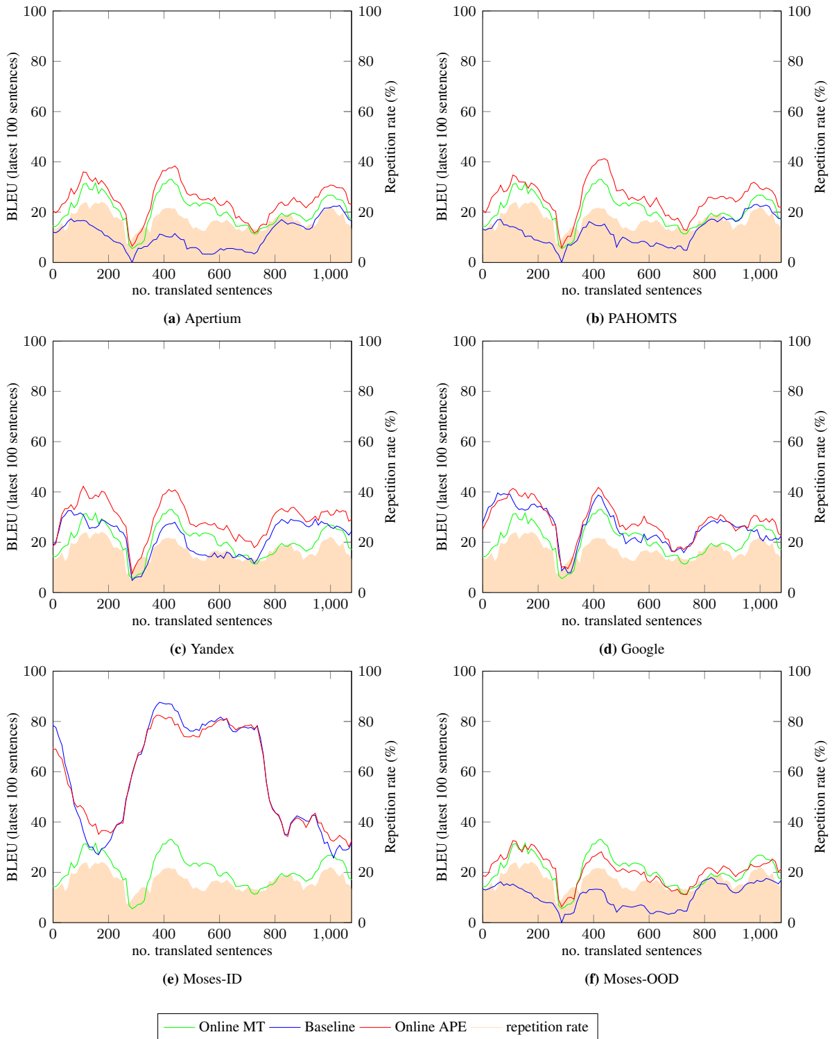
Figure A.14: Dynamics of online learning APE for the Xerox corpus (Spanish to English). The plots show the evolution of BLEU and repetition rate for a window of the latest 100 sentences, as the user completes the translation. The base system is compared to the APE system and a baseline online learning system.
