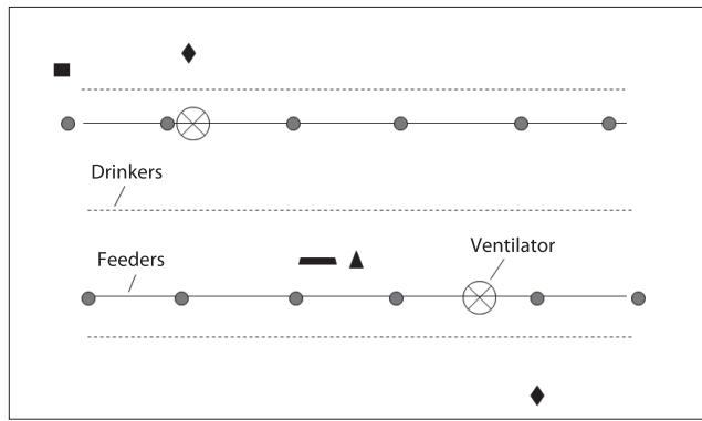
Figure 1. Schematic diagram of a poultry house showing sampling locations (■ Particulate Matter sampler (TEOM); ▬ Andersen cascade impactor; ▲ Impingers; ● Gravitational plates; ◆ Temperature and relative humidity sensors)
