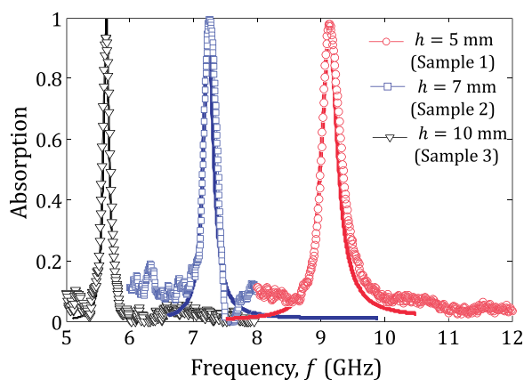
FIG. 4. Absorption spectra for three values of cavity length h . The dielectric thickness is \ell = 1.2 \text{ mm} (slab 1) and the angle of incidence is \theta = 45^\circ . Symbols represent the measurements and continuous lines represent the results obtained with the semi-analytical model.
