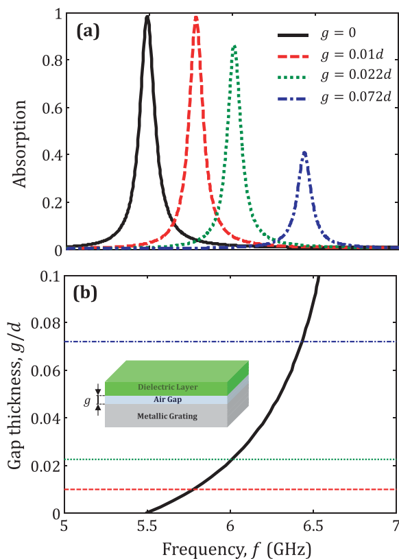
FIG. 3. Effect of non-perfect contact between the dielectric layer and the metallic grating on the frequency of the absorption peak (numerical predictions) for the sample 1 ( h = 10 mm) with the slab 1 ( \ell = 1.2 mm) when the incidence angle is \theta = 45^\circ . (a) Calculated absorption spectra for several values of air gap thickness, g . (b) Calculated position of the absorption peak as a function of the air gap thickness, g . The inset illustrates the structure studied here.
