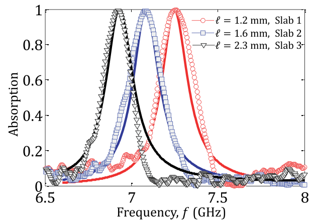
FIG. 5. Absorption for the sample 2 ( h = 7 \text{ mm} ) with three different dielectric thicknesses. The angle of incidence is \theta = 45^\circ . Symbols represent the measurements and solid lines represent the theoretical model.
