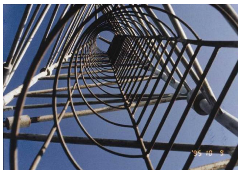
Figure 5: Self-radiating medium-wave mast in solid round bars
