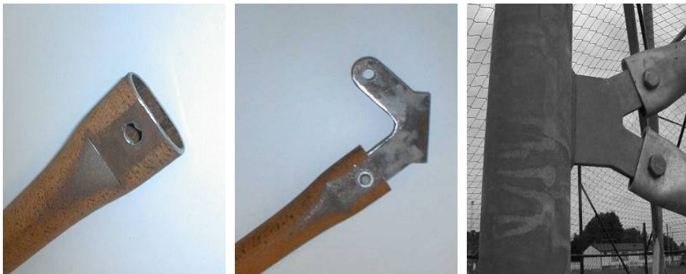
Figure 8: Principles of the assembly of the diagonals
