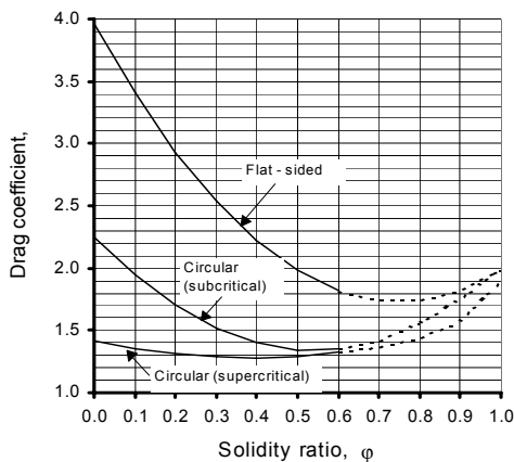
Figure 2: Drag coefficient of square structures
