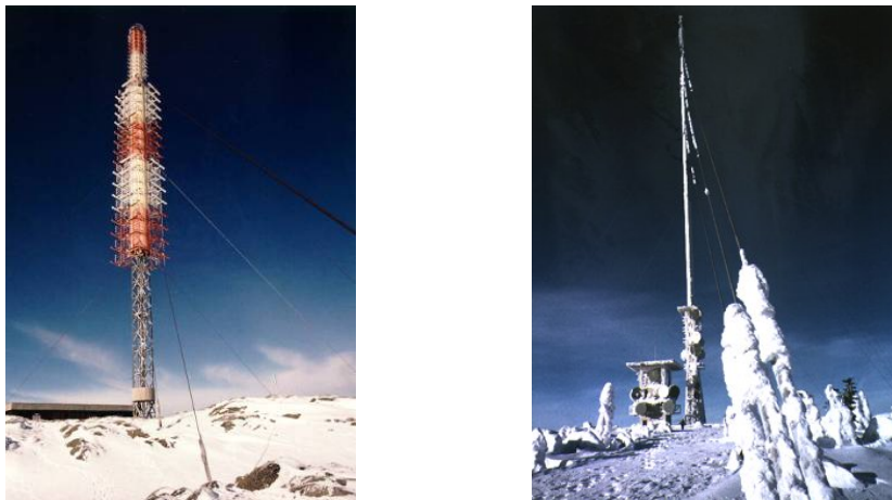
Figure 4: Some masts are so heavily equipped with antennas so the wind resistance of the structure itself is not so important, and some masts are exposed to atmospheric icing which in combination with wind will decide the design.
