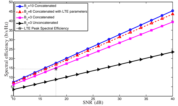
Fig. 2. Spectral efficiency of concatenated and single-channel Grassmannian with M = N = \frac{T_c}{2} = 4 ; LTE peak spectral efficiency also depicted.
