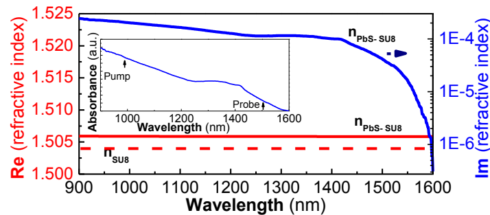
Fig. 2. Real (red solid line) and imaginary (blue solid line) parts of the PbS-SU8 ( ff =0.01) refractive index and real (red dashed line) part of the SU8 refractive index. The inset shows the absorption spectra of the PbS-SU8 QDs at pump (980 nm) and probe (1550 nm) wavelengths.
