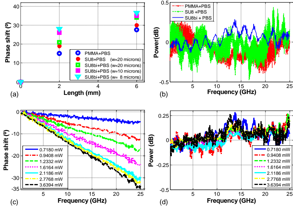
Fig. 4 a) Phase shifting at 25 GHz suffered by the MW signal for different waveguides with different widths and lengths and b) RF amplitude response as a function of the microwave frequency for different waveguides when they are pumped by the 980 nm laser under the highest output power. c) Phase shifting as a function of the microwave frequency and d) amplitude response in the 20 \mu\text{m} wide 6 mm long SU8 bilayer waveguide by pumping with the 980 nm laser for different coupled powers to the input edge of the structure.
