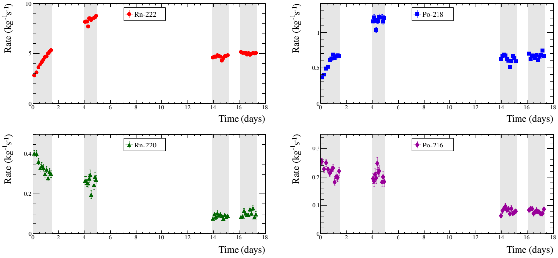
Figure 9. Decay rate versus time for the four alpha-emitting isotopes ^{222}\text{Rn} , ^{218}\text{Po} , ^{220}\text{Rn} , ^{216}\text{Po} . The grey areas with data points correspond to the events used in this analysis, at 0.6, 0.3, 0.8 and 1 kV/cm drift field settings from early to late times, respectively. The time origin is set as the beginning of the 0.6 kV/cm run, approximately one day before the calibration source was inserted. The rate drop between the 0.6 and 0.8 kV/cm runs is due to changes in DAQ conditions.
