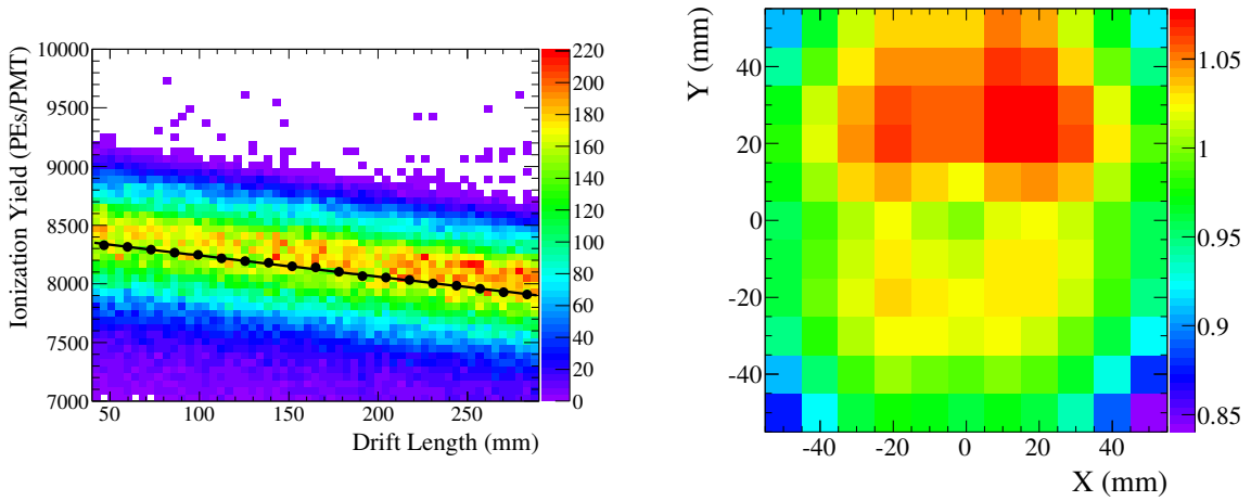
Figure 3. Ionization ( S_2 ) yield of alpha candidate events as a function of spatial position. Left panel: yield (in PEs/PMT) versus drift length ( z -position). Data are fitted to an exponential function, shown by the black curve and accounting for electron attachment. Right panel: yield versus (x, y) position, computed in 10 \text{ mm} \times 10 \text{ mm} wide bins. The yields are normalized to the response on the detector central axis ( x = y = 0 ).
