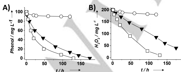
Figure 1. Temporal profiles of phenol degradation (A) and consumed H 2 O 2 (B) using G-based catalysts. Legend: G (□), rGO (▼) and GO (○). Reaction conditions: Catalyst (200 mg L -1 ), phenol (100 mg L -1 , 1.06 mM), H 2 O 2 (200 mg L -1 , 5.88 mM), pH 3, 20 °C.
