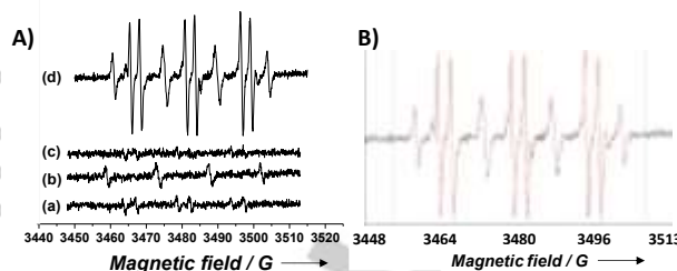
Figure 4. (A) EPR spectra of (a) PBN + H 2 O 2 ; (b) rGO + PBN; (c) PBN + H 2 O 2 ; (d) rGO + H 2 O 2 + PBN. (B) EPR spectra of sample (d) and its fitting (red lines) considering the PBN-OH adduct ( A G N = 15.5 and A G H = 2.7) and tert -butyl aminoxy ( A G N = 14.58 and A G H = 13.90) coinciding with the reported values in the literature. EPR reaction conditions: rGO (200 mg L -1 ), PBN (1,041 mg L -1 , 5.88 mM), PBN to H 2 O 2 molar ratio 1:1, pH 3, 45 min reaction time.
