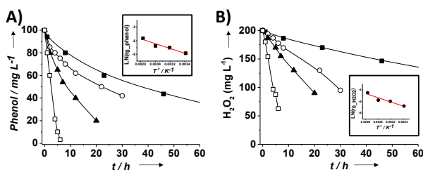
Figure 3. (A) Phenol degradation and (B) \text{H}_2\text{O}_2 decomposition as a function of the reaction temperature using rGO as catalyst. The insets show the Arrhenius plot for both processes. Reaction conditions: Catalyst ( 200 \text{ mg L}^{-1} ), phenol
