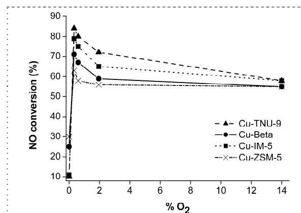
Figure 3. Influence of oxygen concentration on the SCR of NO with propane. (▲) Cu-TNU-9; (●) Cu-Beta; (■) Cu-IM-5; (○) Cu-ZSM-5. Experimental conditions: 700 ppm NO, 390 ppm C 3 H 8 , N 2 as carrier, T= 450 °C, total flow: 900 ml.min -1 , 0.6 gr. of catalyst.
