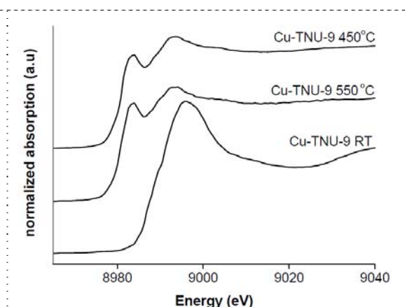
Figure 2. Cu K-edge XANES spectra of Cu-TNU-9 in He at different temperatures of catalyst treatment: RT, 550°C and 450°C.
