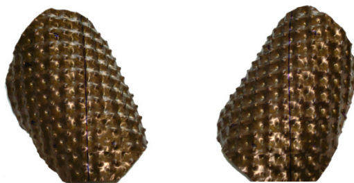
Figure 5: A doubly corrugated shell showing two twisted synclastic stable states.
