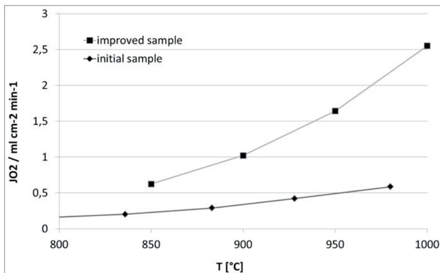
Fig. 5 Permeation tests with a LSCF membranes (feed: air; sweep: argon; at atmospheric pressure)
