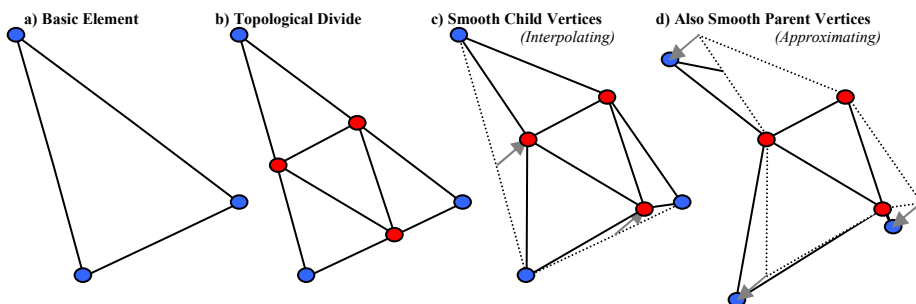
Figure 1: Schematic explanation of subdivision algorithms.
