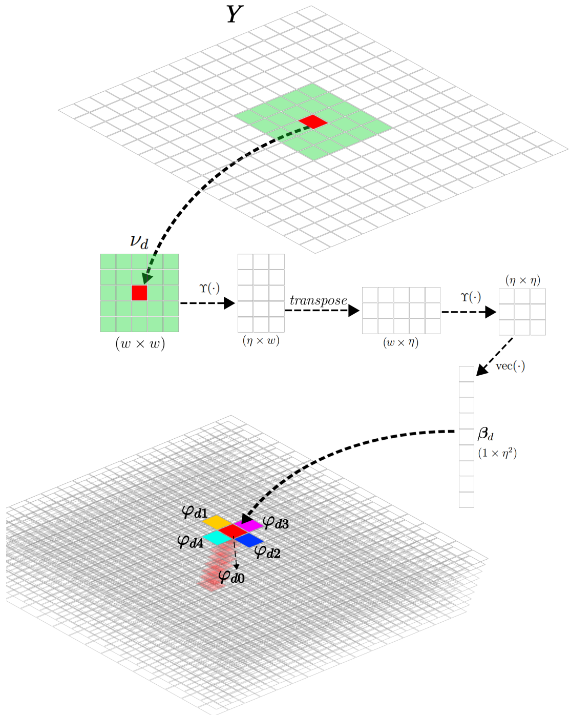
Figure 3.3: Feature extraction process
