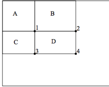
Figure 4.2: The sum of the pixels within rectangle D can be computed with four array references. The value of the Integral Image at location 1 is the sum of the pixels in rectangle A. The value at location 2 is A + B , at location 3 is A + C , and at location 4 is A + B + C + D . The sum within D can be computed as 4 + 1 - (2 + 3) . [8]
