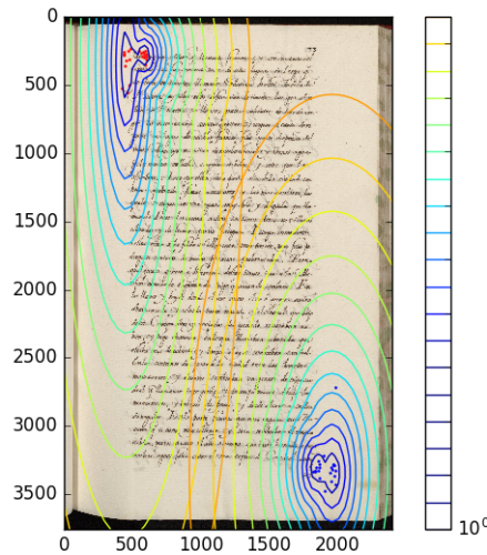
Figure 3.5: Gaussian Mixture Models over main paragraph corners.
