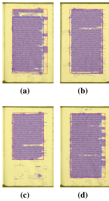
Figure 4.4: CCL results examples, red line. Ground-truth added for reference, blue line. Pages a) 0944, b) 0945, c) 0948 and d) 0958.
