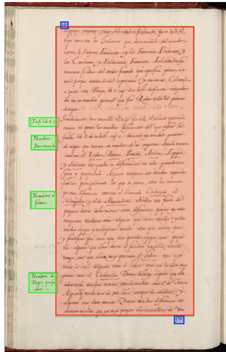
Figure 4.1: PLANTAS layout zones; green for marginalia, red for paragraph, and blue for catch-word.
