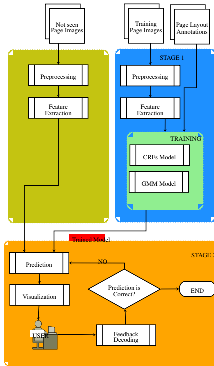
Figure 3.2: System Architecture Diagram.
