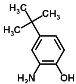
Scheme 1: Chemical structure of 2-amino-4-tert-butylphenol (2A-4TBP)
