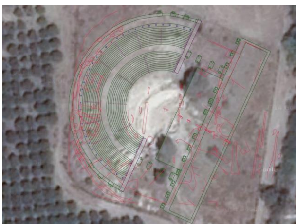
Figure 2: Resulting plan of the large theatre of Gortyn obtained by the combination of architectural elements indicated by Belli, Falkener and Taramelli, according to an orthophoto of the area and the results of geophysical prospection.
