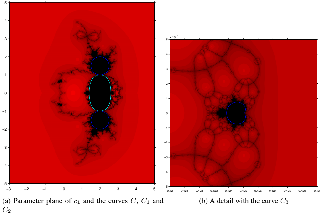
Figure 13: The basins of attraction of z = 1, z_1 and z_2 in the parameter plane of c_1 .
