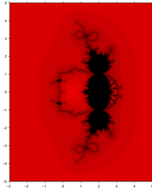
Figure 11: Parameter plane for the critical point c_1 .
