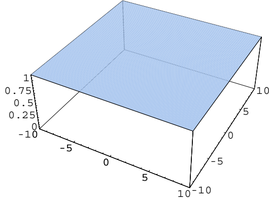
Figure 9: Stability functions for z_3 .
