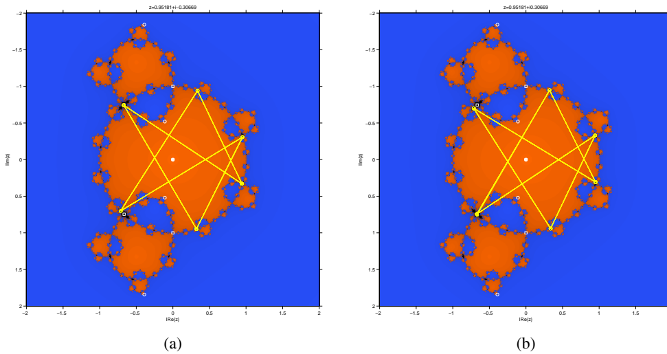
Figure 15: Dynamical plane for a = 1 and periodic orbits of period 6
