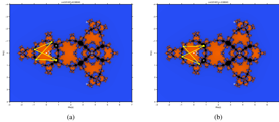
Figure 17: Dynamical plane for a = 3
