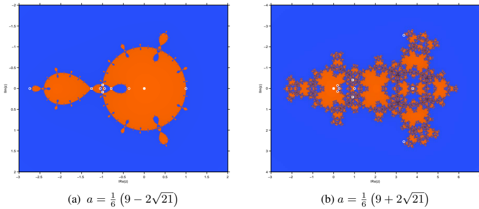
Figure 18: Dynamical planes for a = \frac{1}{6} (9 \pm 2\sqrt{21})
