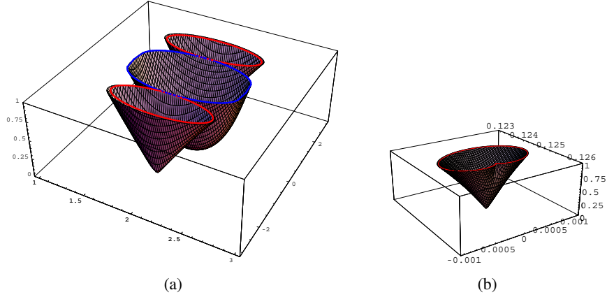
Figure 4: Stability functions of the strange fixed points, z_1, z_2 and z = 1 and the curves C, C_1, C_2 and C_3 in the complex plane.
