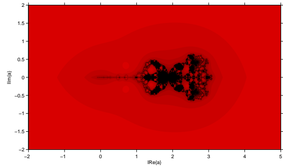
Figure 12: Parameter plane for the critical point c_3 .
