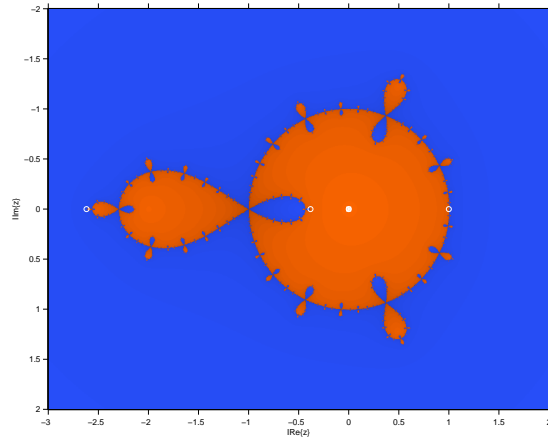
Figure 14: Dynamical plane for a = 0
