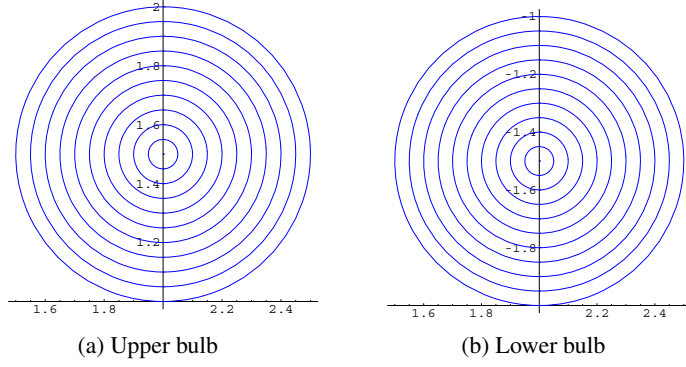
Figure 5: Fiber of circles inside the bulbs
