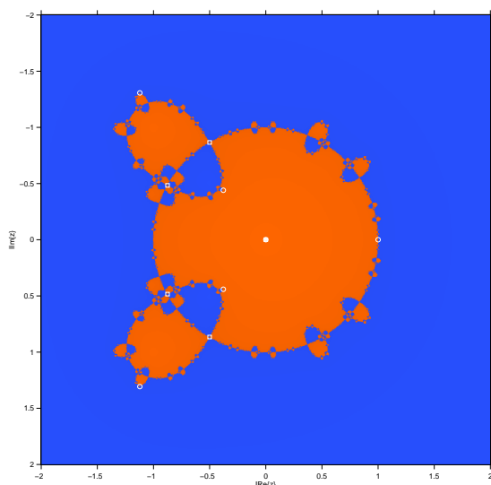
Figure 19: Dynamical plane for a = \frac{1}{2}
