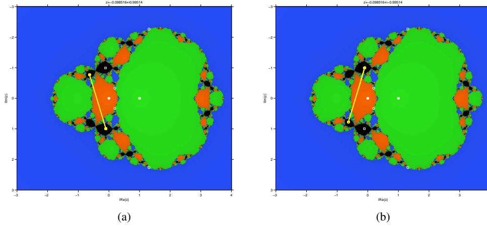
Figure 16: Dynamical plane for a = 2
