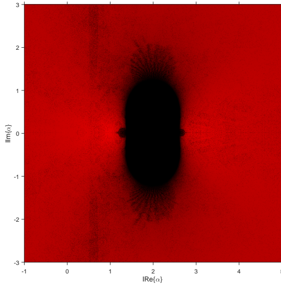
Figure 10: Parameter plane for the critical point c_+
