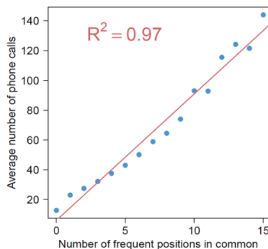
Fig. 6 Correlation between the average number of phone calls between two users and the number of frequent positions in common
