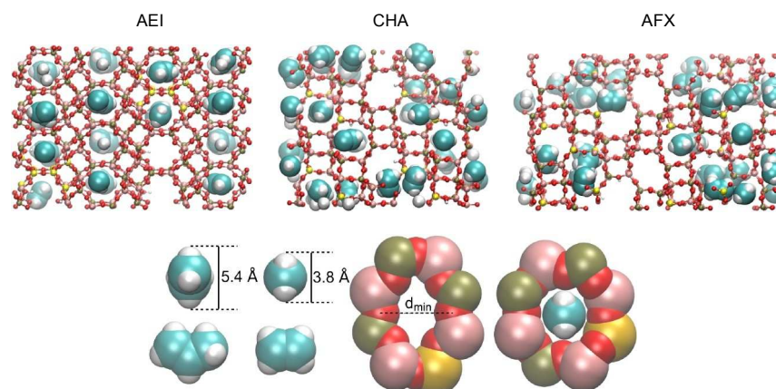
FIG. 1: (Top) Structures of SAP0-18 (AEI), SAP0-34 (CHA), and SAP0-56 (AFX), loaded with ethene molecules. (Bottom left) Van der Waals representations of ethene and propene in front and side orientations. (Bottom middle) An elliptically shaped 8-ring with indicated d_{min} distance. The ring is too small for ethene to cross through. (Bottom right) An 8-ring with more circular shape that is large enough for ethene to cross through. Atom colors: C (blue), H (white), O (red), Al (pink), Si (yellow), P (taupe).
