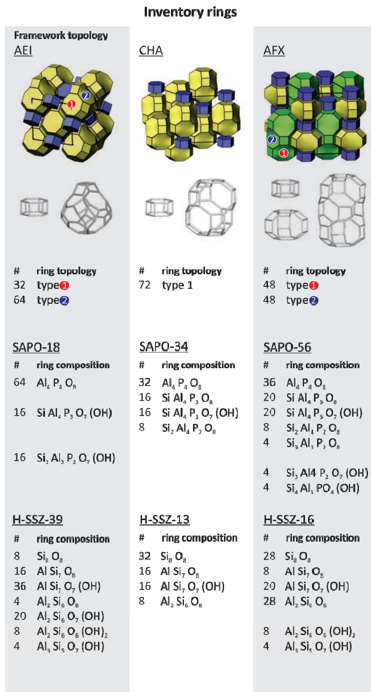
FIG. 4: Inventory of rings according to ring topology and ring composition (ring character). Top part of figure is adapted from IZA database. 2
