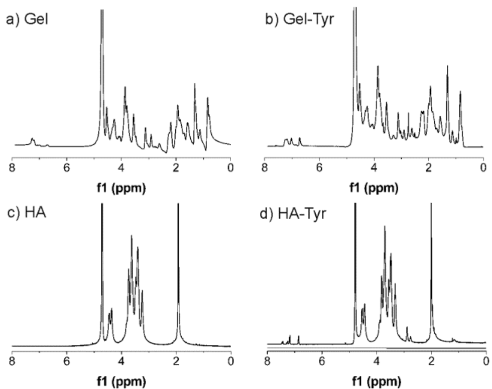
Figure S1. 1 H-NMR spectra of a) gelatin, b) tyramine grafted gelatin, c) hyaluronic acid and d) tyramine grafted HA.
