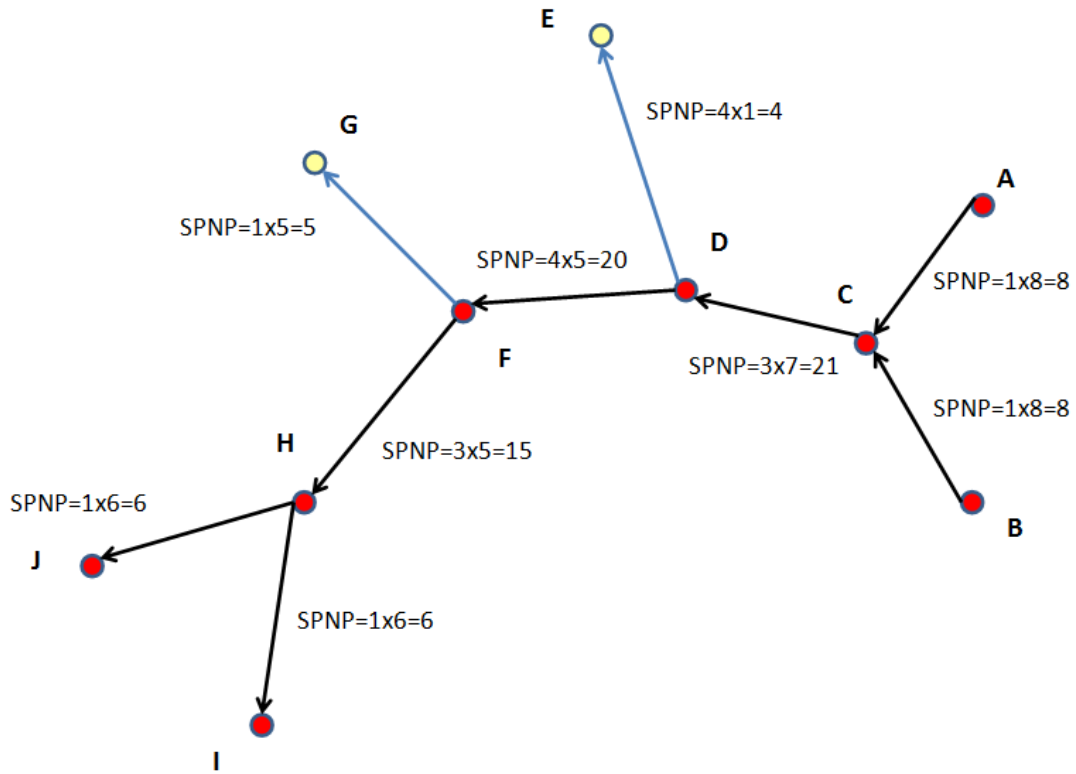
Figure 1. Calculation of SPNP. The main path is in black.
