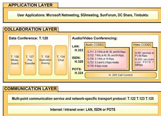
Figure 4. Architecture of communication tools.
