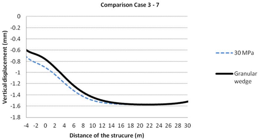
Figure 16: Vertical displacements in Case 3 and Case 7
