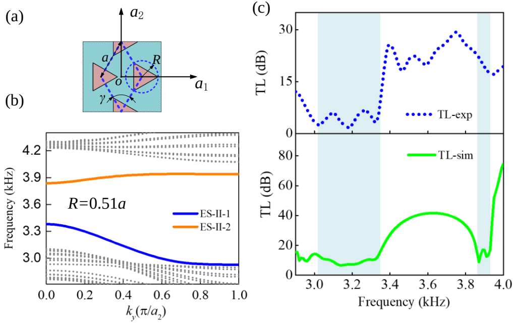
FIG. 17. (a) Scheme of the unit cell. The distance between rods is a , and the radius of the outer circle of the triangular rods is R . (b) The dispersion relation of the supercell containing Interface II with R = 0.51a . The gray dots represent bulk modes. The blue and orange lines represent the bands ES-II-1 and ES-II-2 composed of topological states, respectively. (c) Transmission loss (TL) obtained from experiments (upper panel) and numerical calculations (bottom panel). The green line represents the numerical simulations in the inviscid approximation. Shaded regions define the bandwidth of bands ES-II-1 and ES-II-2.
