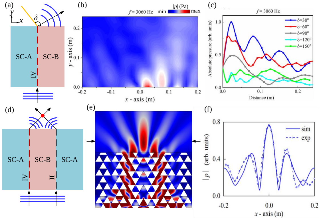
FIG. 18. (a) Schematic diagram representing the propagation of a planar wavefront impinging a structure containing the Interface IV. The horizontal blue lines represent the impinging wavefront; the red dotted line represents the excited edge state while the arrow, which forms an angle of \delta with the x-axis, represents the main propagation direction. (b) Snapshot of the absolute pressure map measured in the scanned area using
