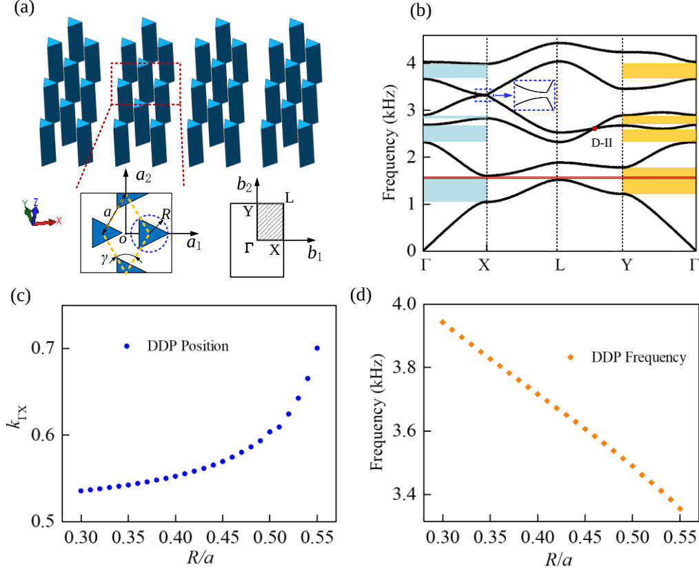
FIG. 1. (a) 3D view of Suzuki phase crystal under study. One of the two insets shows a zoom view of the 2D unit cell with the lattice vectors \mathbf{a}_1 and \mathbf{a}_2 . The centers of the four triangular cylinders whose circumcircle radius is R form a rhombus with side length a , and the rhombus angle \gamma is 60^\circ . In addition, the center of the rhombus coincides with the center of the Suzuki phase cell at point O. The other inset shows the FBZ of the Suzuki phase, where vectors \mathbf{b}_1 and \mathbf{b}_2 are the lattice vectors of the reciprocal lattice and the rectangle \Gamma XLY define the irreducible BZ. (b) Dispersion relation of an ASP cell. The blue shading indicates the bandgap in the \Gamma X direction, and the yellow area indicates the bandgap in the \Gamma Y direction. Red shading indicates the complete bandgap. Dotted boxes indicate zoomed-in views of bands near point X. (c) The relationship between the position of DDP in k -space and the ratio of R/a . Since the length ratio of \Gamma X and XL is 0.75: \sqrt{3}/2 , the relative length of \Gamma X is 0.75 when the relative length of XL is taken as \sqrt{3}/2 . (d) The relationship between the frequency of DDP and the ratio of R/a .
