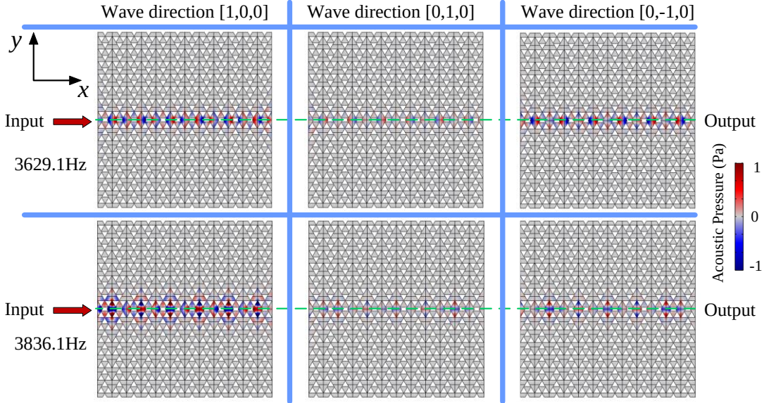
FIG. 12. Sound transmission along Interface III with impinging waves coming from different directions with frequencies corresponding to edge states A_1 ( A_1' ) and B_1 ( B_1' ).
