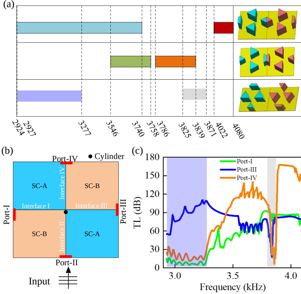
FIG. 16. (a) Frequency spectra of the topologically protected edge states. (b) Scheme of a SC structure made of SC-A and SC-B containing the four interfaces. (c) The transmission spectra for waves transmit through a path composed of different Interfaces. The green line, blue line, and orange line represent the transmission spectra of Port-I, Port-III, and Port-IV, respectively. The blue (gray) shadow stripe represents the frequency interval of the edge states on Interface II (IV).
