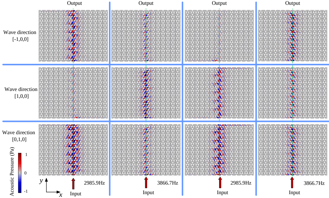
FIG. 13. Snapshots of the sound transmission along Interface II (IV) produced by plane waves with different incident directions. The frequencies correspond to edge states A_3 ( A_4 ) and B_3 ( B_4 ).
