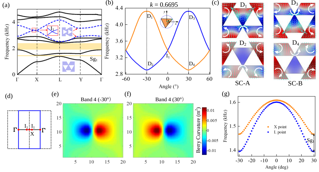
FIG. 3. (a) Band structure for the ASP lattice with R=0.54a . The solid lines indicate dispersion relation with \beta=30^\circ (see the inset the bottom). The dashed lines depict the fourth and fifth bands obtained with the unit cell shown in the top inset, where the triangular rods are rotated 0^\circ . The yellow stripes indicate the complete bandgaps, where Sg_1 denotes the lowest frequency bandgap. (b) Dependence on the rod rotation angle ( \beta ) of the frequency of the quasi-type-II DP. The blue and orange solid lines represent the two modes involved in the DP. The inset defines the rotation angle \beta . (c) Pressure patterns of modes obtained when rods are rotated \pm 30^\circ . Red and blue colors denote positive and negative values, respectively. The white circular arrows represent the flux of acoustic energy. (d) The FBZ of the ASP lattice. The dotted rectangles indicate two adjacent FBZs, and the solid line rectangle indicates the FBZ constructed from the center \Gamma point of two adjacent FBZs. (e) and (f) show the Berry curvature distribution of the 4 th band for the rotation angles -30^\circ and +30^\circ respectively. (g) Rotation dependence of the frequencies at the L point of the 1 st band (blue dotted line) and at the X point of the 2 nd band (orange dotted line). The separation between both frequencies defines the bandgap width Sg_1 .
