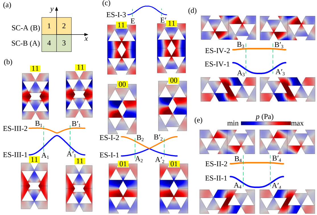
FIG. 5. (a) Scheme of the structure containing SC-A and SC-B. The SC is divided into four regions, 1 to 4, where four different interfaces can be formed. (b) Snapshots of the sound pressure pattern of the edge states located at Interface III (calculated at k_x = 0.5 and 1.5 , respectively). The numbers enlightened in yellow represent the mirror symmetry about the xz -plane and yz -plane, respectively, “1” means symmetric, and “0” means anti-symmetric. The blue and orange lines provide the dispersion relation of the edge modes. (c) Snapshots of the sound pressure pattern of the edge state located along Interface I. The upper panel corresponds to eigenmodes at k_x = 0.1 and 1.9 , and the middle and lower panels represent eigenmodes at k_x = 0.5 and 1.5 . (d) and (e) depict the sound pressure patterns of edge states at interfaces IV and II respectively. The color scale represents the magnitude of the magnitude of the real component of the pressure, going from negative values (blue) to positive values (red).
