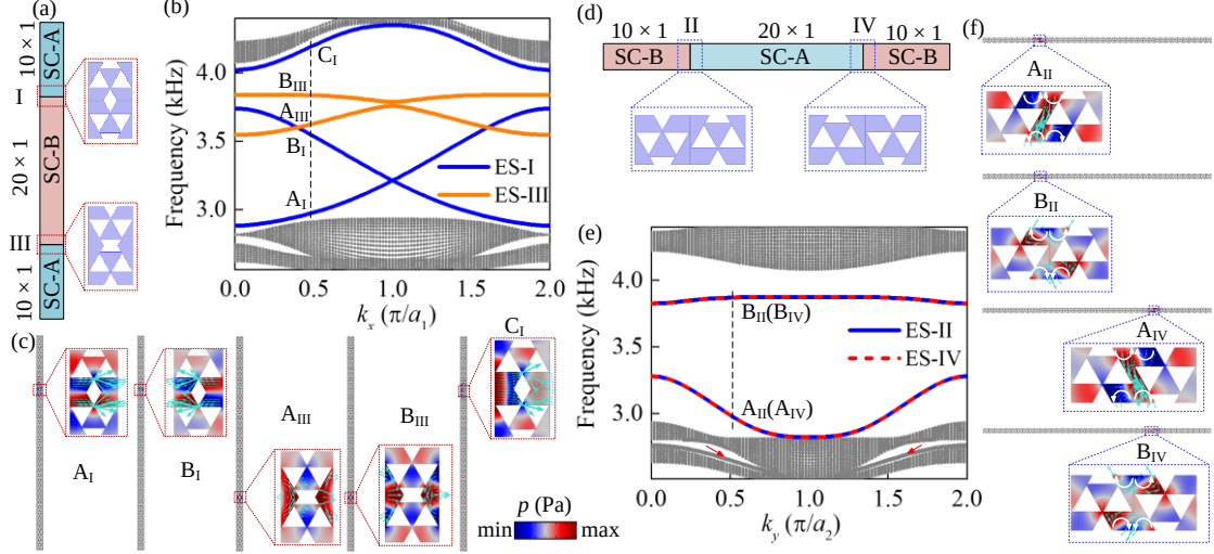
FIG. 4. (a) Scheme of the superlattice composed of SC-A and SC-B with Interface I and Interface III. The red-dotted rectangular box displays a zoomed view of interfaces I and III. (b) Acoustic band structure of the supercell (a) around the quasi-type-II DP. The black dots represent bulk bands. The blue and orange lines represent the edge states located on interfaces I and III, respectively. (c) Acoustic pressure patterns and energy flow of eigenmodes A_I , B_I , and C_I at Interface I, and A_{III} and B_{III} at Interface III at k_x = 0.5 . (d) Scheme of the superlattices obtained by combining SC-A and SC-B. Their respective interfaces are denominated as Interface II and Interface IV. The blue dotted rectangles show zoom views of the two interfaces. (e) Band structure the supercell containing interfaces II and IV, where the dotted lines represent bulk modes. The blue lines (ES-II) and red dashed lines (ES-IV) represent the edge states located at Interface II and Interface IV, respectively. (f) Pressure patterns and energy flow distribution of the eigenstates denominated A_{II} , B_{II} , A_{IV} , and B_{IV} . The colored maps represent the acoustic pressure (real part) and the cyan arrows represent the energy flux.
