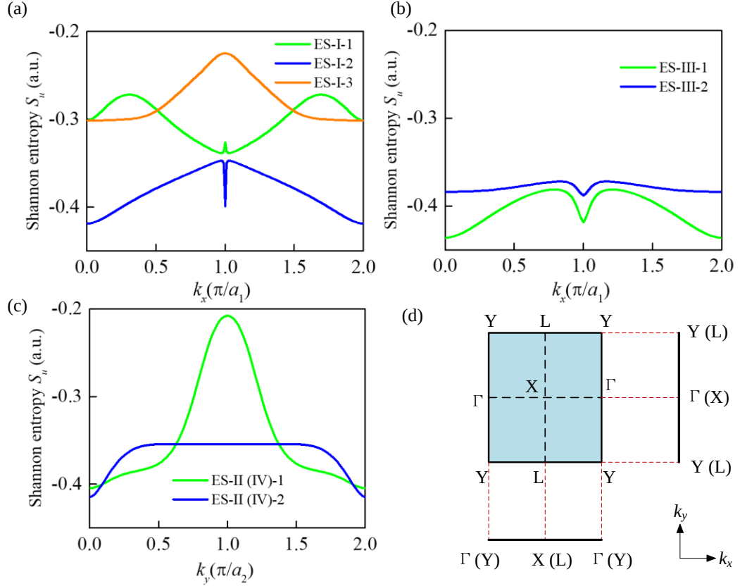
FIG. 6. (a) Acoustic Shannon entropy of eigenmodes localized at Interface I. Green, blue and orange lines represent topologically protected edge states ES-I-1, ES-I-2, and ES-I-3, respectively. (b) Acoustic Shannon entropy corresponding to eigenmodes localized at Interface III. Green and blue lines represent the edge states ES-III-1 and ES-III-2, respectively. (c) Acoustic Shannon entropy corresponding to eigenmodes localized at Interface II(IV). Green and blue lines represent the edge states ES-II(IV)-1 and ES-II(IV)-2, respectively (d) 1D projection of the vector of the 2D first BZ of the Suzuki phase in the k_x and k_y directions, respectively.
