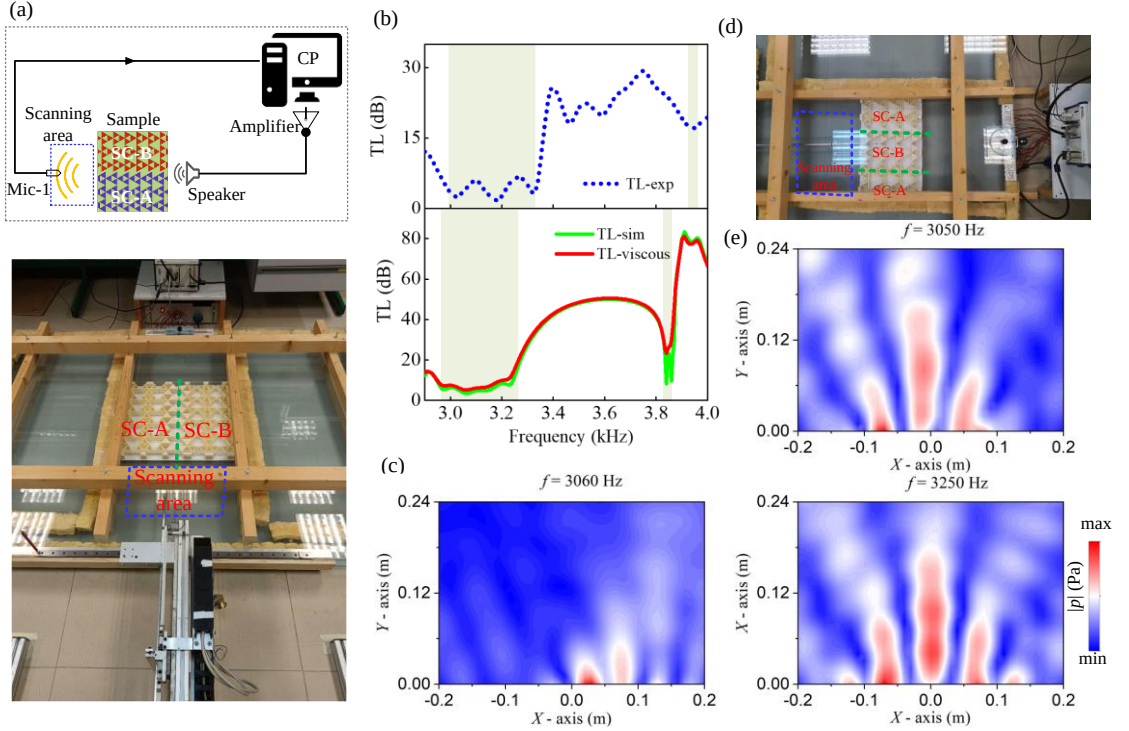
FIG. 8. (a) Experiment setup. The top panel and bottom panel show the scheme of the data acquisition process and scene photo, respectively. (b) Transmission loss (TL) calculated (bottom panel) and measured (upper panel). The red and green lines define the TL obtained with and without thermal viscous losses, respectively. The blue-dotted line represents the TL obtained from measurements. The shadowed areas define the bandwidth of the edge states. (c) The absolute pressure pattern at the scanning area was obtained experimentally. (d) Experiment setup for acoustic focusing. (e) Absolute pressure distribution in the scanning area was obtained experimentally at 3050Hz (top panel) and 3250Hz (bottom panel). Color represents the absolute pressure.
