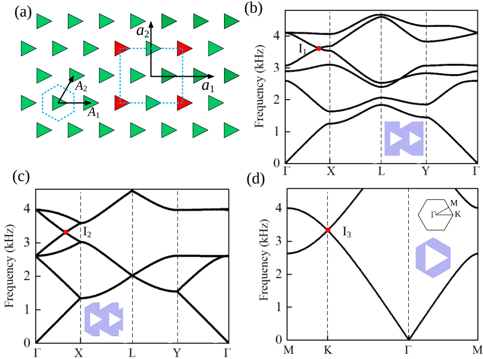
FIG. 9. (a) Schematic diagram of a sonic crystal consisting of scatterers with triangular section distributed in a triangular lattice. The blue dashed hexagon
