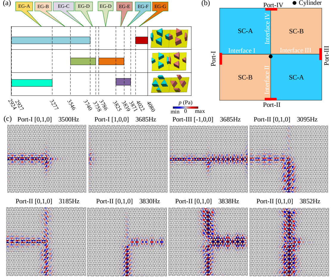
FIG. 7. (a) Frequency spectra of the topologically protected edge states. The 1st row indicates the frequencies of states (blue and red strips) of supercell containing interface I. The 2nd row defines frequencies (green and orange strips) with states localized at interface III. The cyan and magenta strips in the 3rd row indicate the frequencies of edge states localized at interface II or IV. The bands are further divided into seven smaller frequency bands (defined on top) according to overlapping features. (b) Scheme of a SC structure made of SC-A and SC-B containing the four interfaces. The distinct edge states are excited through ports named I, II, III, and IV. The black dot indicates the auxiliary cylinder employed to disturb the field of the impinging waves arriving at the ports. (c) Propagation of a plane-wave with direction [0, 1, 0] at 3500Hz from Port-I, with direction [1, 0, 0] at 3685Hz from Port-I, with direction [-1, 0, 0] at 3685Hz from Port-III, with directions [0, 1, 0] at 3095Hz from Port-II, with directions [0, 1, 0] at 3185Hz from Port-II, with directions [0, 1, 0] at 3830 Hz from Port-II, with directions [0, 1, 0] at 3838 Hz from Port-II, and with directions [0, 1, 0] at 3852 Hz from Port-II, respectively.
