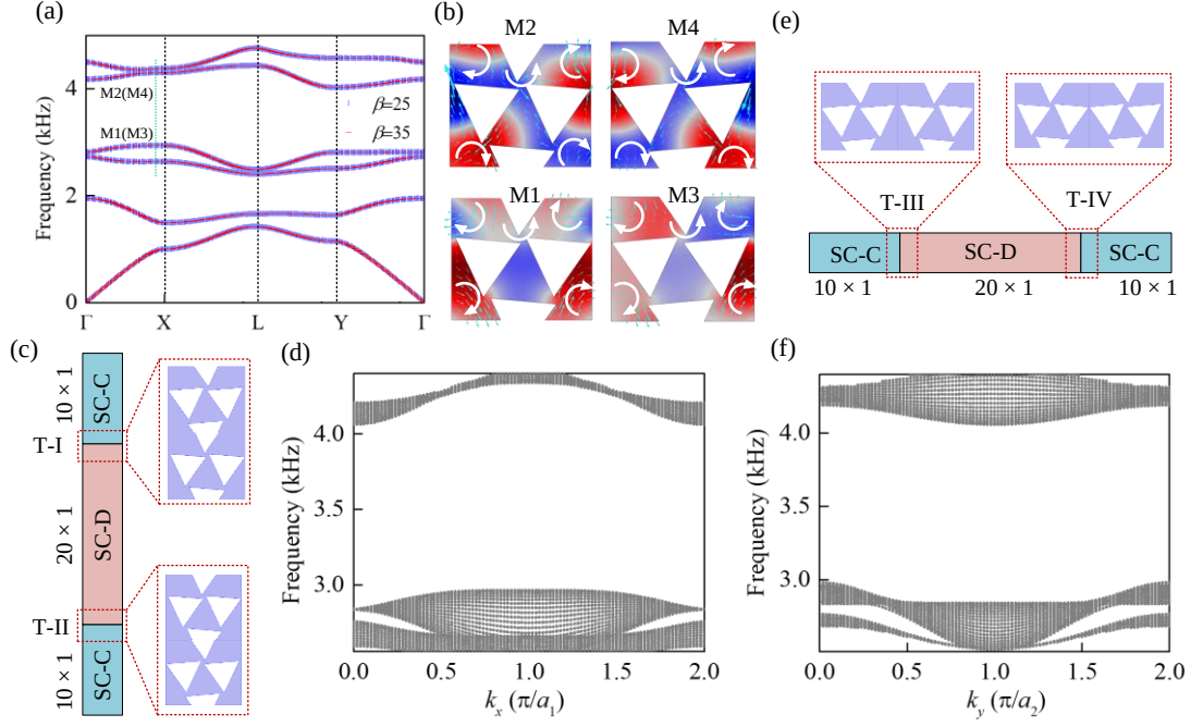
FIG. 10. (a) Band structure with different rotation angles. The blue vertical short line and the red horizontal short line represent the band structure when the rotation angle \beta=25^\circ and \beta=35^\circ , respectively. The green dotted line indicates k=0.6695 , and the intersection of SC with the fourth and fifth bands at an angle of rotation of 25^\circ ( 35^\circ ) is indicated by M1 (M3) and M2 (M4). (b) Sound pressure mode of the states M1-M4. The color represents the sound pressure (real part), in which red and blue colors represent the positive and negative values, respectively. The cyan arrow indicates the sound intensity, and the white circular arrow indicates the direction of the sound energy flow. (c) Scheme of the superlattice composed of SC-C and SC-D with interfaces T-I and T-II. The red-dotted rectangular box deploys a zoomed view of the interfaces T-I and T-II. (d) Projected band structure of the supercell (c) around the double degenerate point. The black dots represent bulk bands. (e) Scheme of the superlattice composed of SC-C and SC-D with interfaces T-III and T-IV. The red dotted rectangular box deploys a zoomed view of the interfaces T-III and T-IV. (f) Band structure of the supercell (e) around the double degenerate point.
