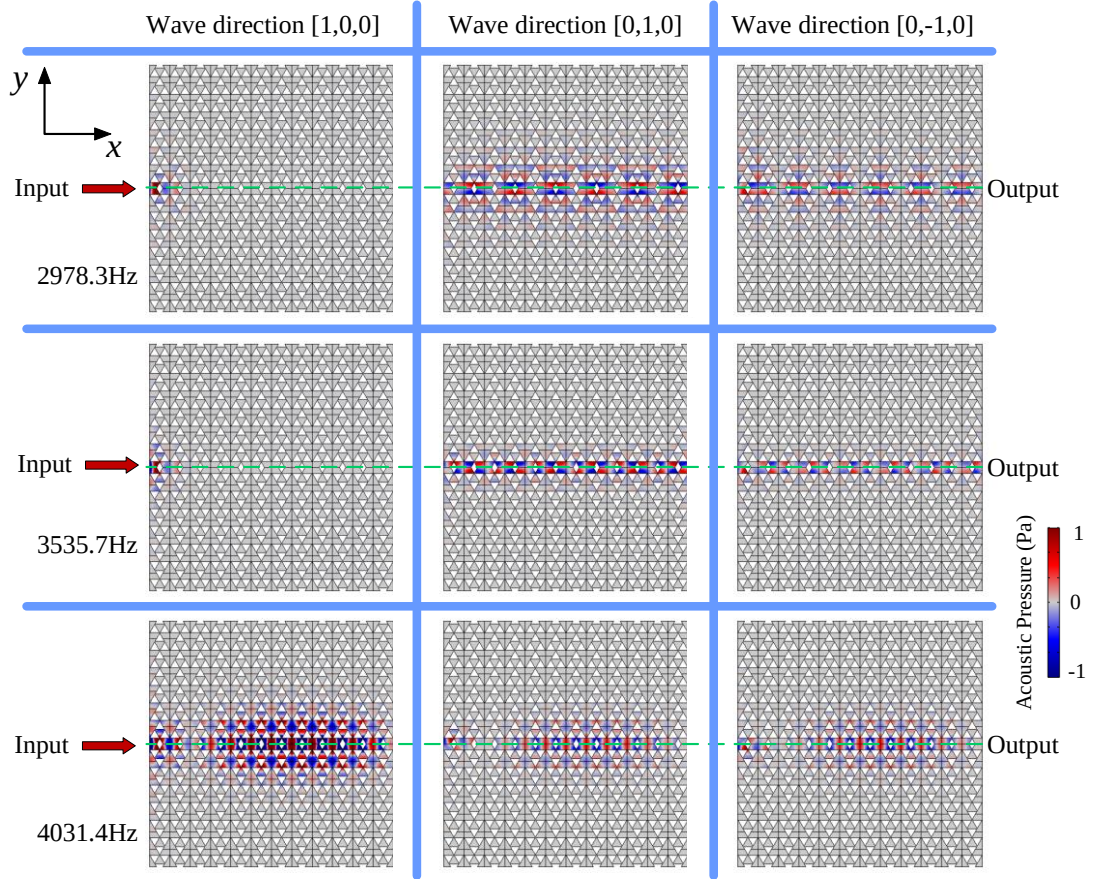
FIG. 11. Transmission of incident waves with different wave vector directions incident on the sound field domain containing Interface I at the frequencies of edge states A_2 ( A_2' ), B_2 ( B_2' ) and E
