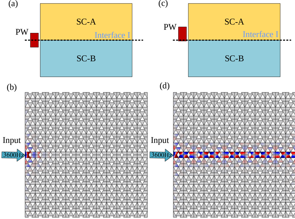
FIG. 14. (a) Scheme of the structure defining Interface I where the exciting beam (PW) is symmetric with respect to the interface. (b) Snapshot of the total pressure pattern obtained with the previous configuration when the incident beam has frequency 3600 Hz (c) Scheme of the structure defining Interface I where the exciting beam (PW) is non-symmetric with respect to the interface. (d) Snapshot of the total pressure obtained with the previous configuration at the frequency of 3600 Hz. Now the deaf edge mode has been excited due to the asymmetry of the impinging beam.
