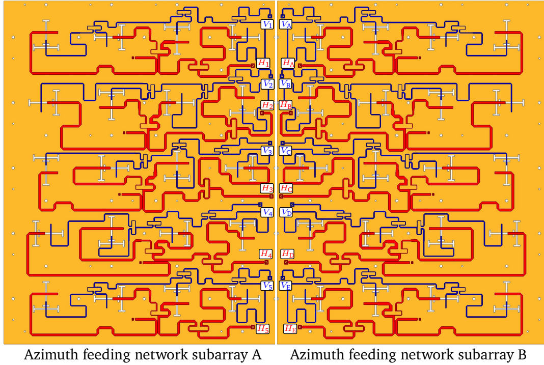
Figure 5.43.: Azimuth feeding network for subarray A and B.
