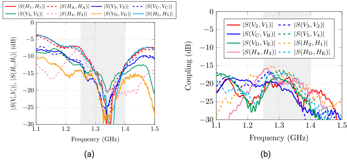
Figure 5.55.: Measured S-parameters of the final array 5×8 prototype at the azimuth feeding network. (a) Reflection factor. (b) Coupling.
