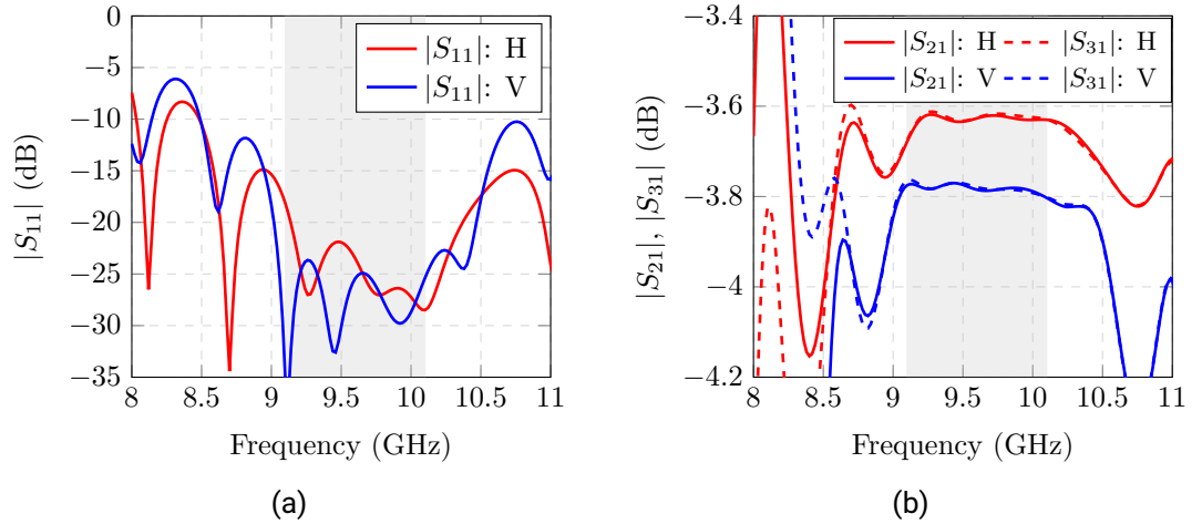
Figure 3.14.: Simulation results power divider H and V: (a) Reflection factor. (b) Transmission factor.
