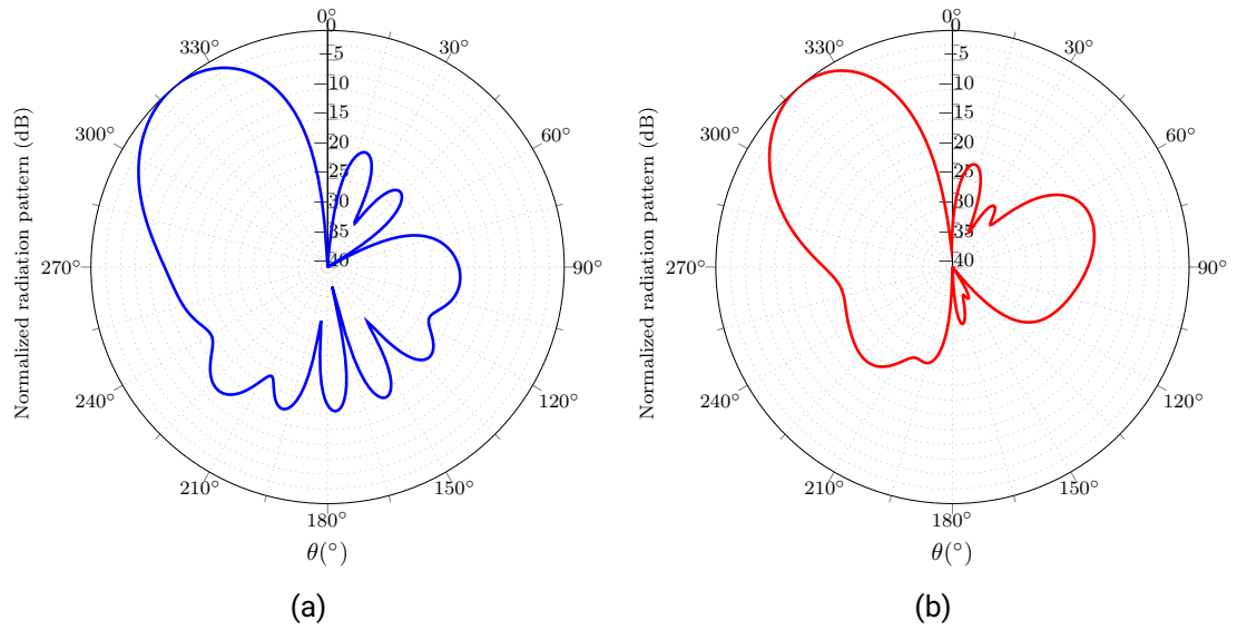
Figure 5.44.: Simulated radiation pattern in elevation of the final array 5×8. (a) Vertical polarization. (b) Horizontal polarization.
