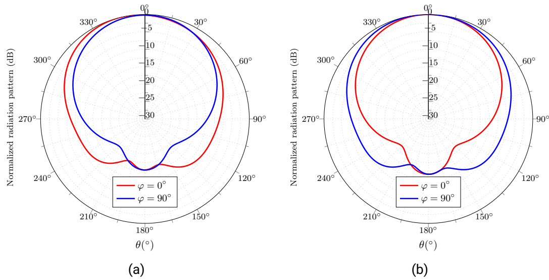
Figure 5.11.: Simulated main cuts of the radiation pattern. (a) Vertical polarization. (b) Horizontal polarization.
