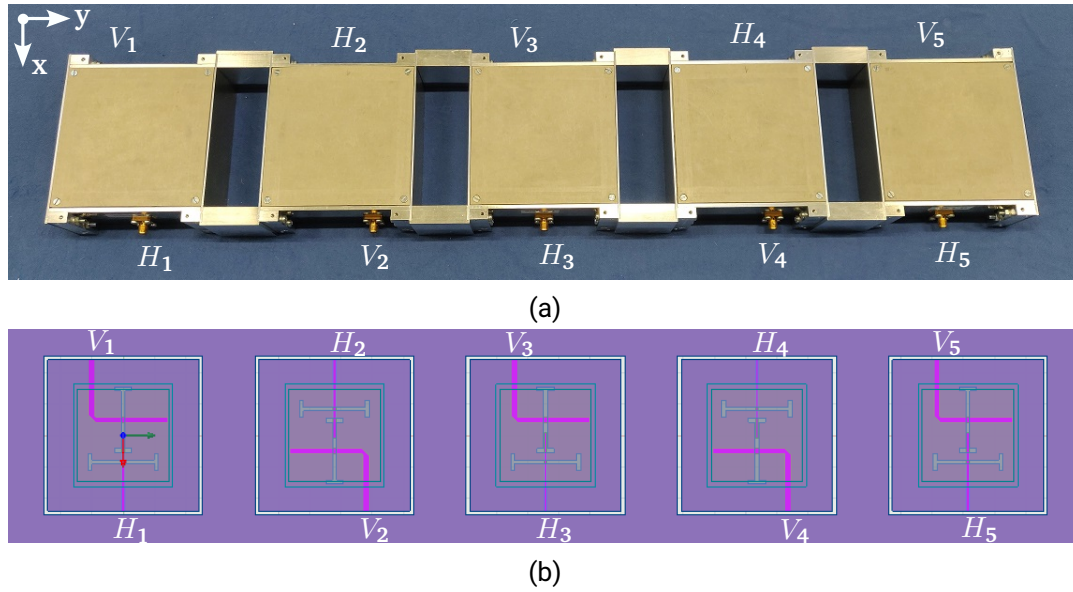
Figure 4.40.: (a) Geometrical arrangement of the linear array with sequential 180° rotation of the antenna elements. (b) HFSS model.
