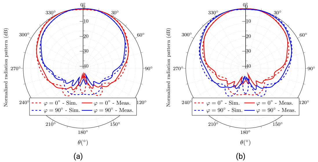
Figure 4.32.: Measured radiation pattern of the antenna prototype and comparison with simulation. (a) Horizontal polarization. (b) Vertical polarization.
