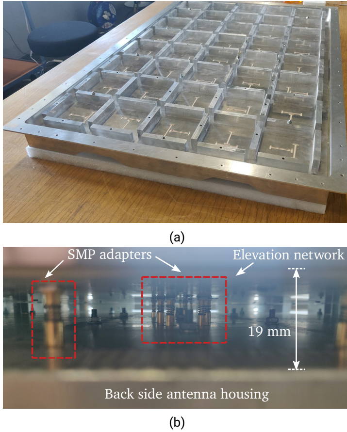
Figure 5.57.: (a) Antenna housing without array elements. (b) View of the SMP adapters.
