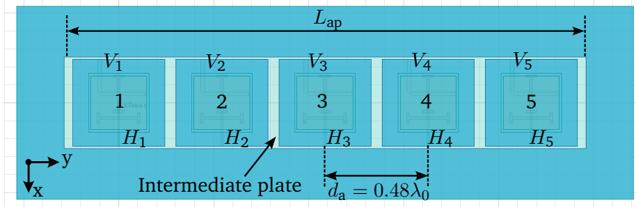
Figure 4.24.: Linear array of 5 cavity-box stacked patches along y-axis. HFSS model.
