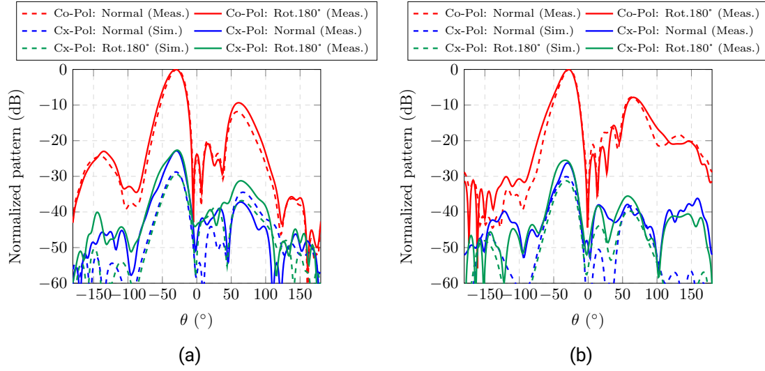
Figure 4.42.: Comparison simulation and measurement of the 180° rotation array. Beam steering. (a) Horizontal polarization. (b) Vertical polarization.
