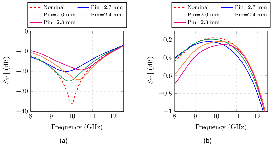
Figure 3.20.: Tolerance analysis connector pin length: (a) Reflection factor. (b) Transmission factor.
