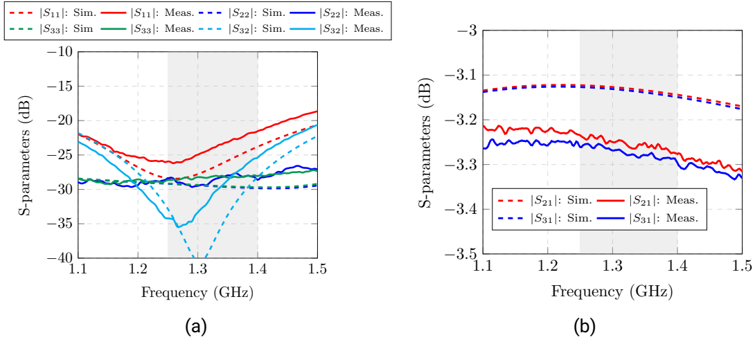
Figure C.11.: Measured S-parameters of the balanced Wilkinson divider V. (a) Reflection factor and output ports isolation. (b) Transmission factor.
