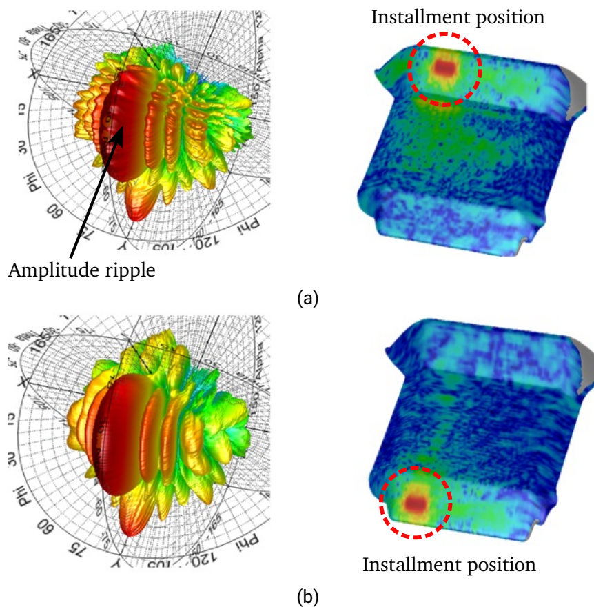
Figure 6.4.: Measured interaction with the carrier depending on the antenna installment position. F-SAR system. (a) Top side. (b) Bottom side.
