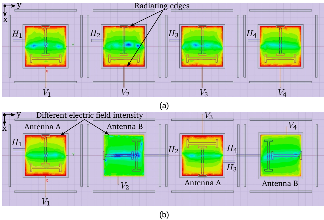
Figure 5.16.: Magnitude of the electric field on the top patches with equal amplitude and phase. Vertical pol. (a) Standard array arrangement with antenna element A. (b) Sequential 90° rotation of array elements combining antennas A and B.
