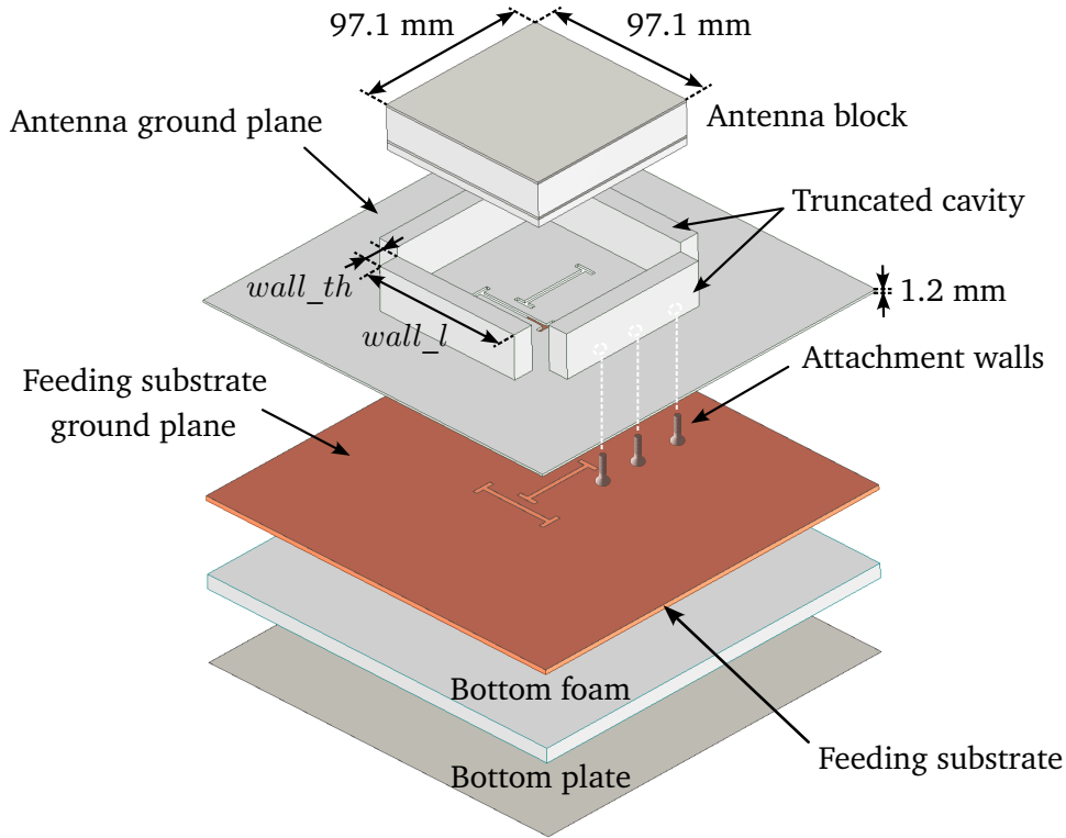
Figure 5.6.: Truncated assembly.
