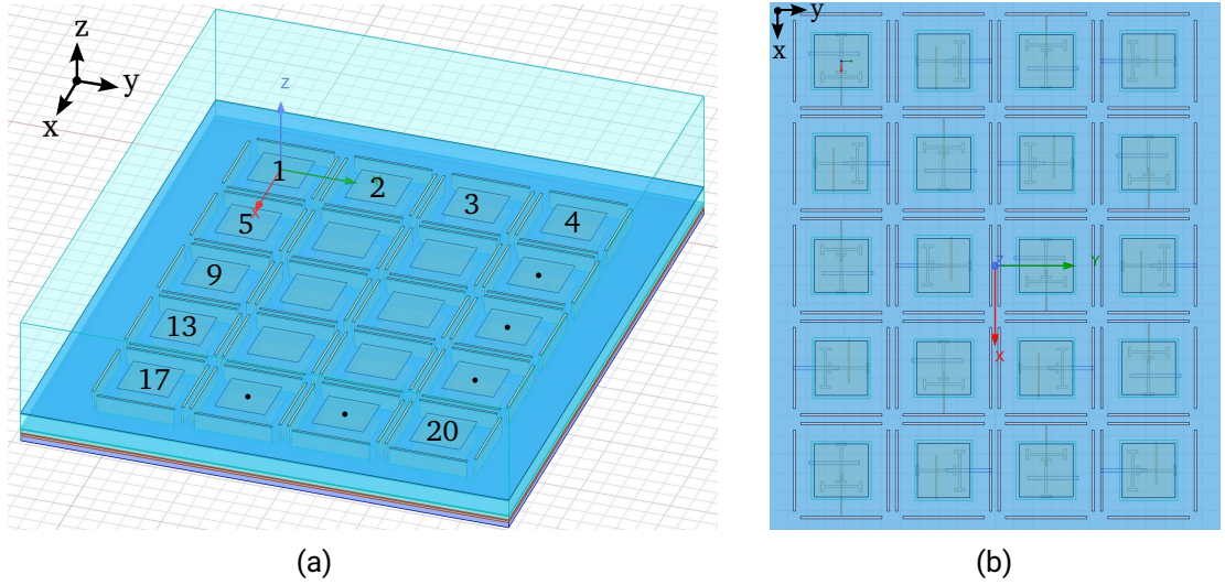
Figure 5.26.: (a) Simulated HFSS model of the subarray 5 \times 4 with element numeration. (b) Top view with the slots arrangement.
