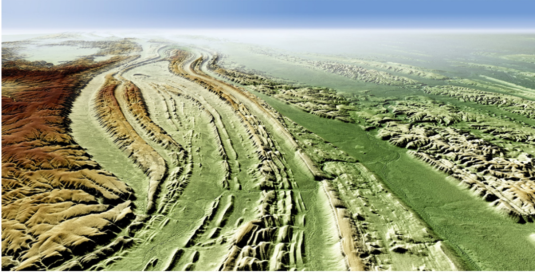
Figure 2.9.: Digital elevation model of Finke Gorge National Park (Australia). Data acquired from TerraSAR-X and TanDEM-X.
