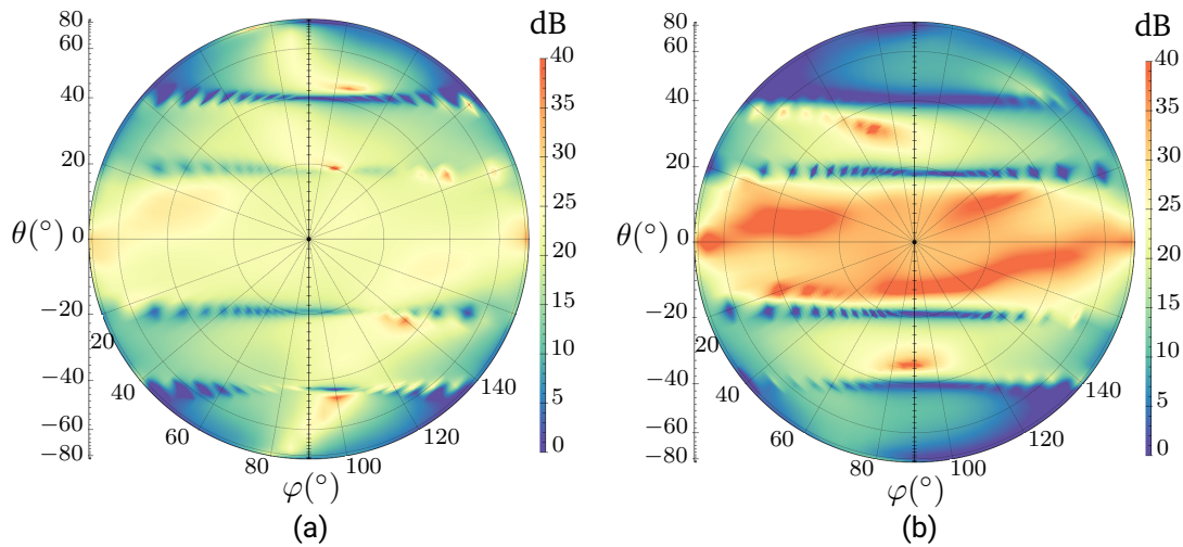
Figure 4.45.: Measured cross-polar suppression values. Horizontal polarization. (a) Normal array. (b) Rotation 90°.
