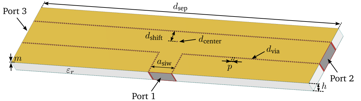
Figure 3.8.: SIW T-Junction model.
