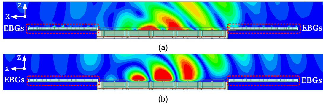
Figure 6.26.: Propagation of the electric fields in elevation with the antenna carrier and EBGs. (a) Vertical polarization. (b) Horizontal polarization.
