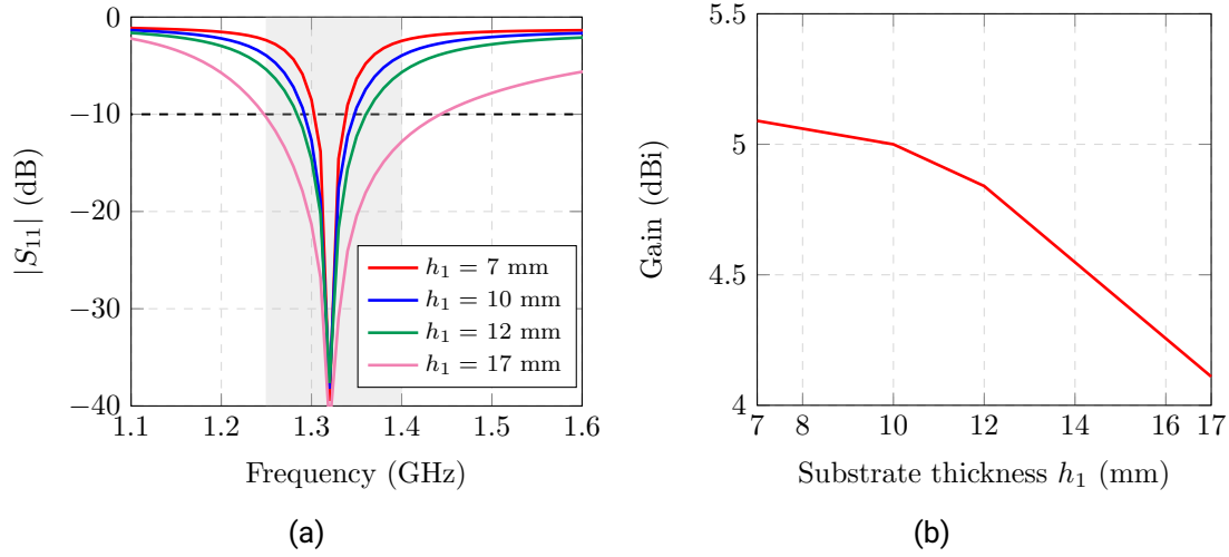
Figure 4.7.: Performance of aperture coupled antenna with dielectric permittivity of the patch substrate \varepsilon_{r_1} = 6.15 (a) Bandwidth (b) Gain @ f_0 = 1.325 GHz.
