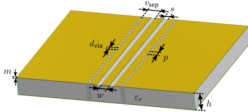
Figure 3.23.: GCPW line.
