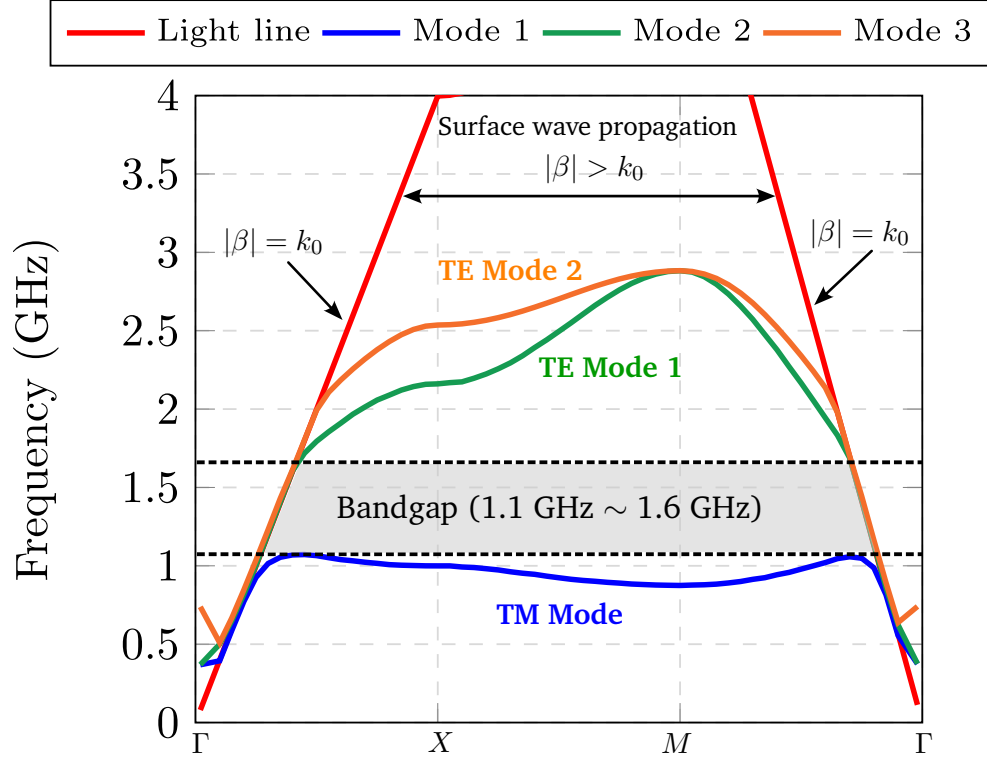
Figure 6.17.: Dispersion diagram.
