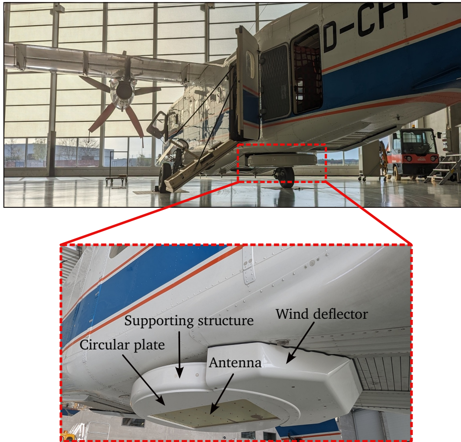
Figure 2.13.: DuoLIM antenna carrier. The attachment position is under the aircraft.
