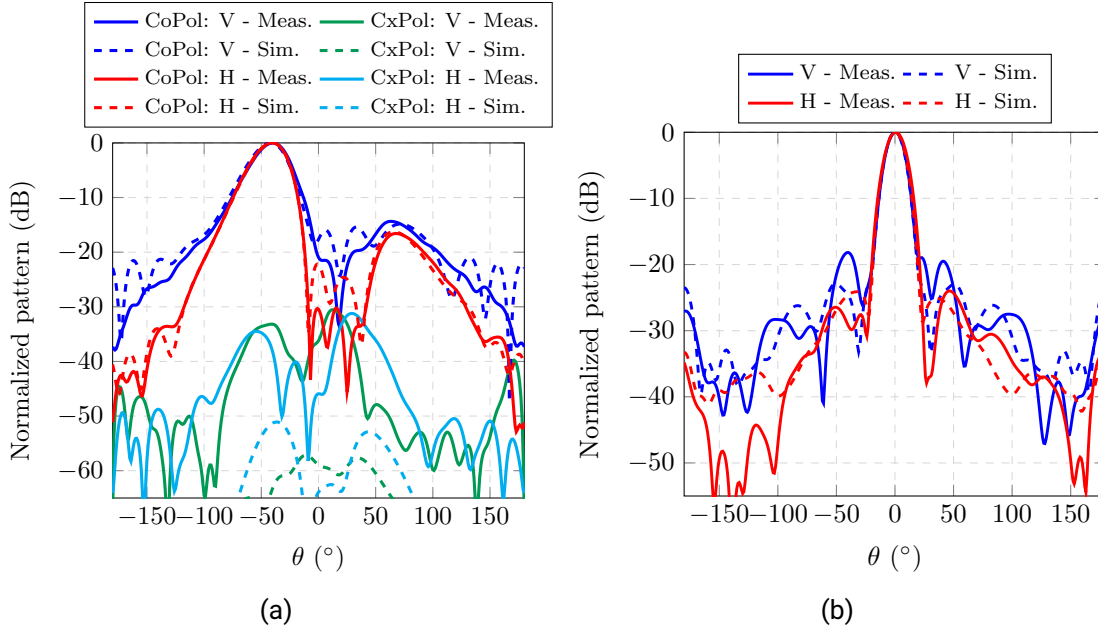
Figure 5.60.: Measured normalized patterns of the final constructed array 5×8 prototype. (a) Elevation. (b) Azimuth.
