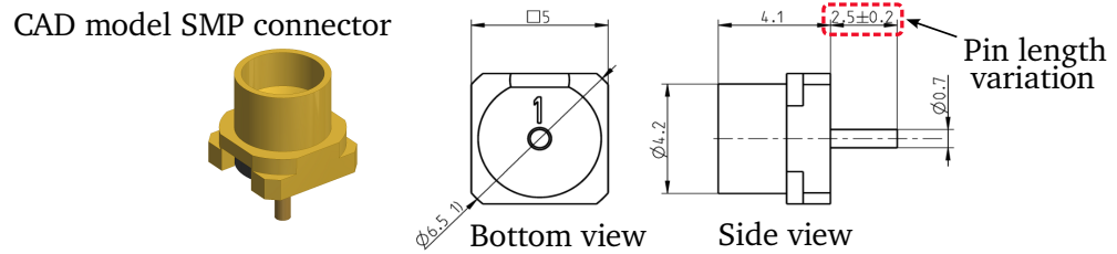
Figure 3.19.: Fabrication tolerances. Possible variation of the connector's pin length.
