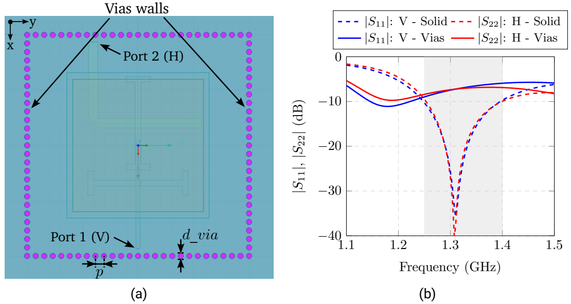
Figure 5.3.: Cavity walls replacement by means of vias. (a) HFSS model. (b) Comparison of the reflection factor with the closed cavity-box.
