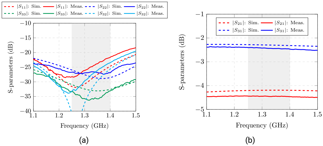
Figure C.12.: Measured S-parameters of the unbalanced Wilkinson divider V. (a) Reflection factor and output ports isolation. (b) Transmission factor.
