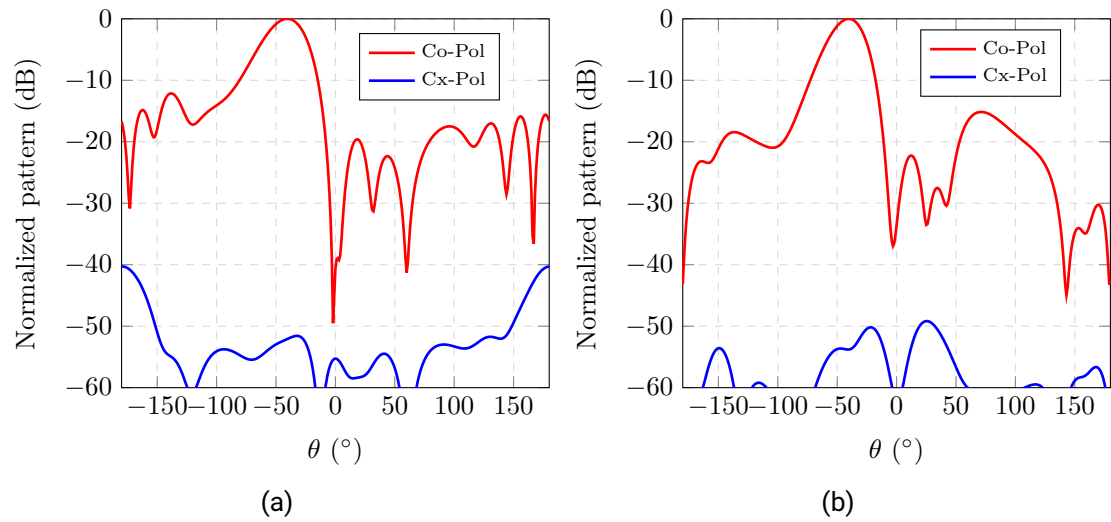
Figure 5.45.: Normalized co-polar and cross-polar patterns in elevation of the final array 5×8. (a) Vertical polarization. (b) Horizontal polarization.
