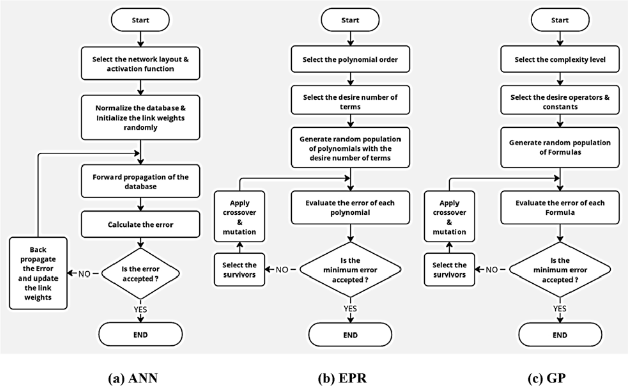
FIGURE 3 Flowcharts for different (AI) predictive models. (A) for ANN, (B) for EPR, (C) for GP.
