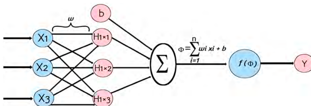
FIGURE 5 Architectural framework of the ANNs.
