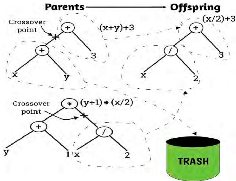
FIGURE 4 Genetic framework of the GP.
