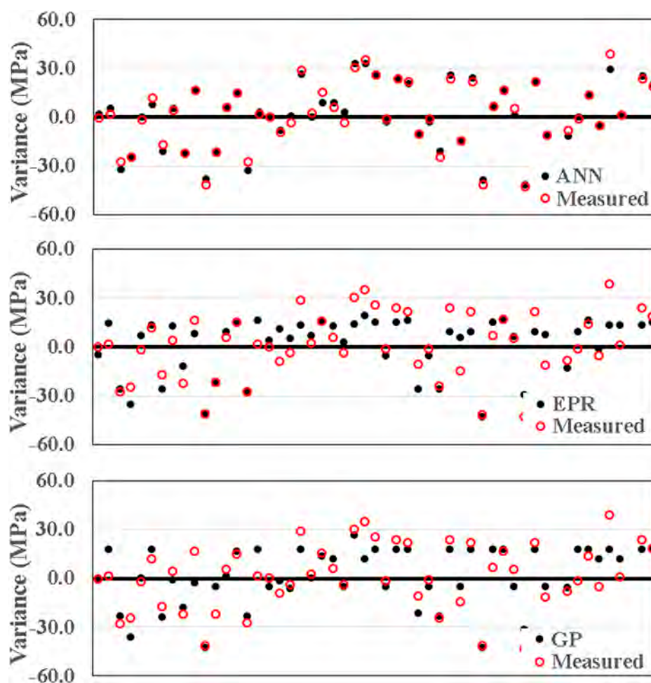
FIGURE 12 Variance distribution for the developed models.
