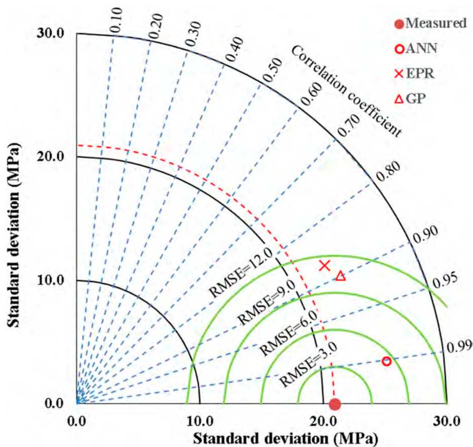
FIGURE 11 Comparing the accuracies of the developed models using Taylor charts.
