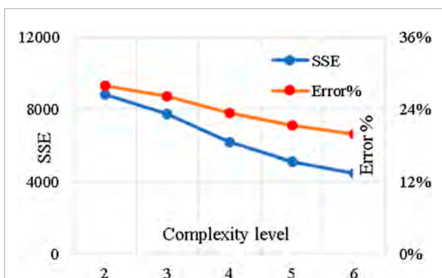
FIGURE 6 GP Model accuracy versus complexity level.
