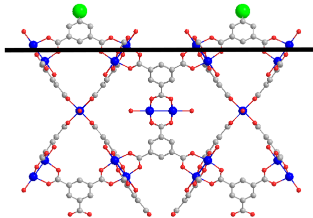
Fig. 4 Structure of HKUST-1 viewed along the \langle 110 \rangle direction, showing the most likely surface termination at the \{111\} faces. The green spheres represent the dangling hydroxy groups of OH-IP linkers pointing outwards from the triangular faces of the octahedral crystals, while the broad black line represents the terminations of these triangular \{111\} faces.
