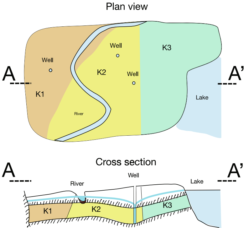
Fig. 1 Aquifer sketch in plan view and cross section
