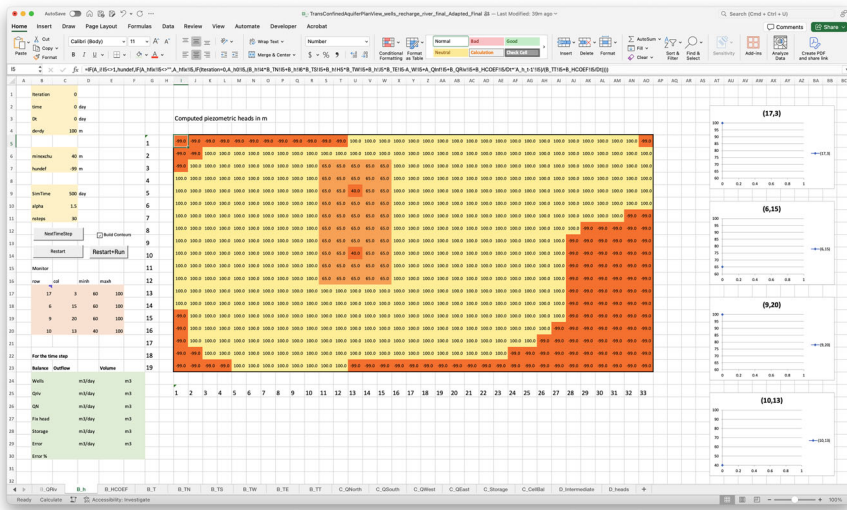
Fig. 5 Sheet B_h after simulation reset. This sheet shows the named variables, the calculated heads for the current iteration and the piezometric head evolution for the observation cells. The buttons that trigger the reset of the simulation, the advance to the next step, and the simulation run along the toggle box to compute the contour plots are also shown
