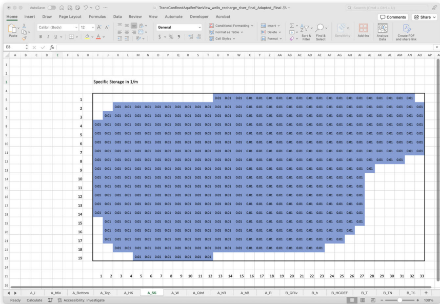
Fig. 3 Specific storage
