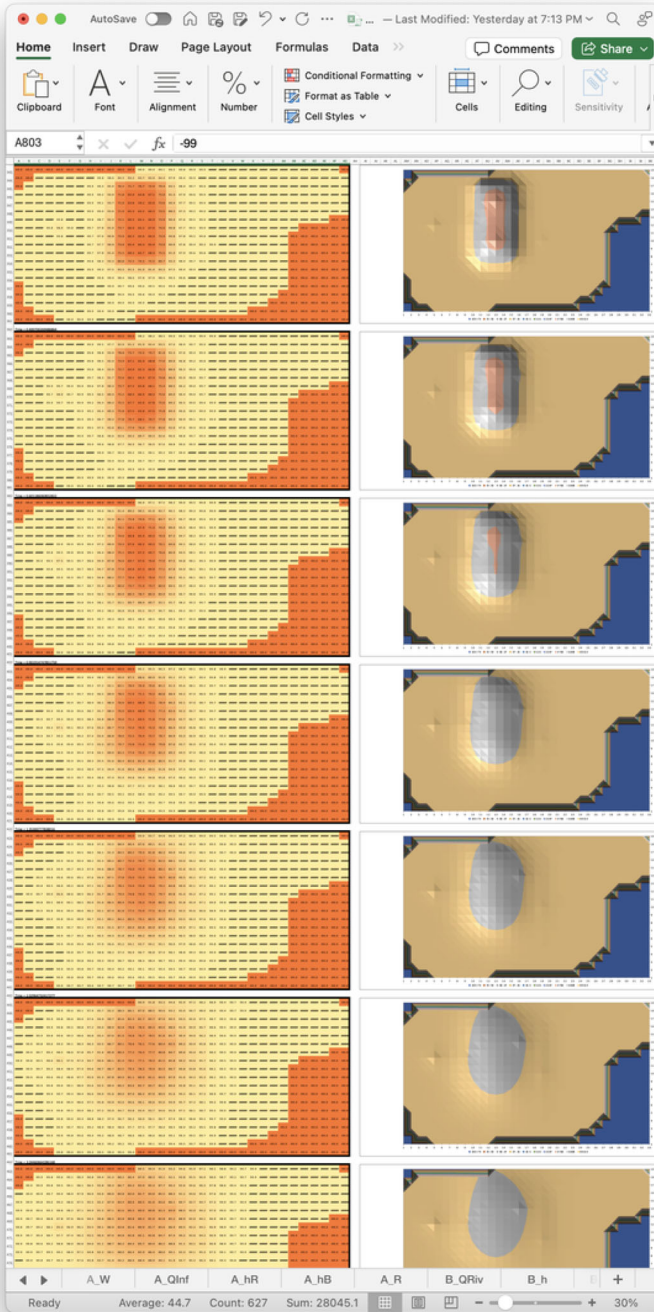
Fig. 8 A glimpse at sheet D_heads where the piezometric head maps are gathered and contoured. Maps shown correspond to times 0.27, 0.40, 0.60, 0.90, 1.35, 2.03, and 3.00 days
