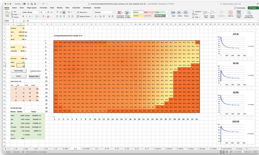
Fig. 7 Heads at t = 3,000 days, approaching steady-state
