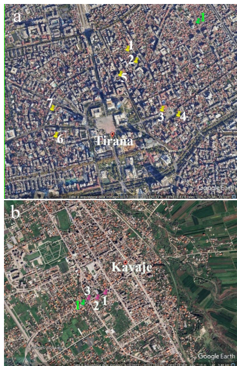
Fig. 4 – Localization of sampled buildings (yellow and dark pink) and soils (green) in Tirana (a) and Kavaje (b) (Edited from Google Earth, 2023).
