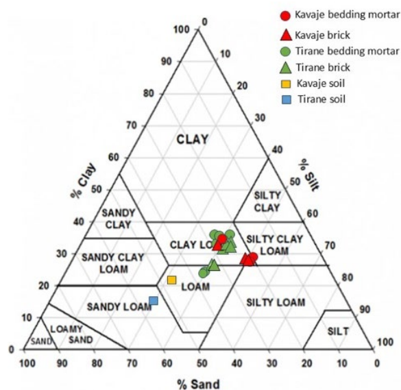
Fig. 12 – Sand-Silt-Clay ternary diagram, showing the grain size composition of building materials and earthen soils (Modified from FAO, 2006).
