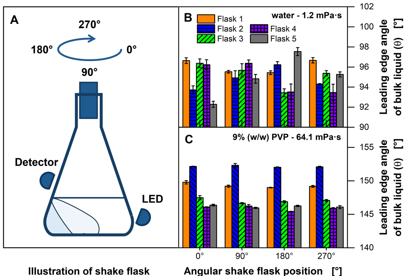
Fig. 2 Determination of leading edge angle of bulk liquid \theta by transmitted light measurement for five shake flasks with varying orientation. (A) Schematic representation of the 90° stepwise rotation and measurement of the shake flask along its longitudinal axis. (B) Shake flasks filled with water (1.2 mPa·s). (C) Shake flasks filled with 9% (w/w) PVP (64.1 mPa·s). (B & C) LED angle: 121°, detector angle: 55°. V_F = 250 mL, V_L = 20 mL, n = 350 min -1 , d_0 = 50 mm, T = 30 °C. Error bars represent the standard deviation of triplicates. Parts of this figure have been adapted from Sieben (2017) [72]
