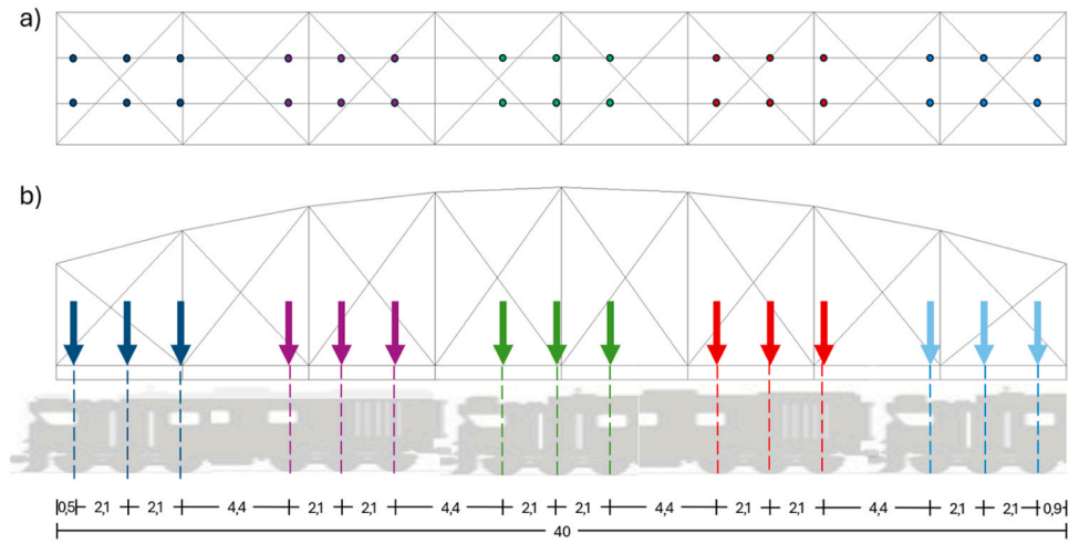
Fig. 5. Critical load position in the steel truss bridge, measurements in meters. (a) Plan view (b) Lateral view.
