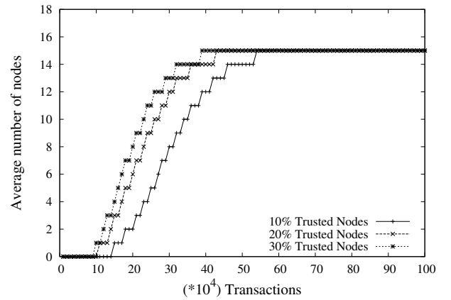
FIGURE 5. Size of the trustset on non trusted nodes
