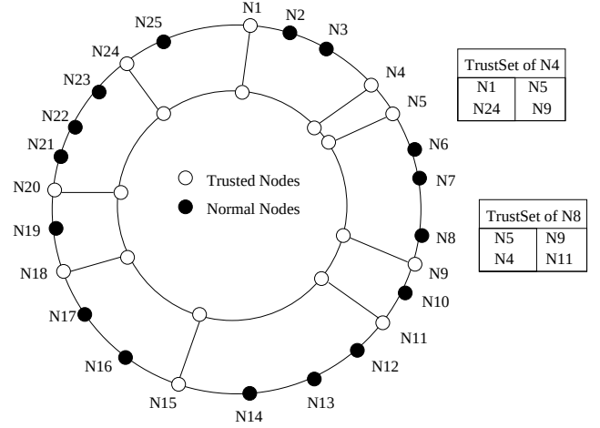
FIGURE 2. Example of trustset structure
