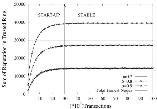
FIGURE 8. Convergence of the Trusted Ring size
