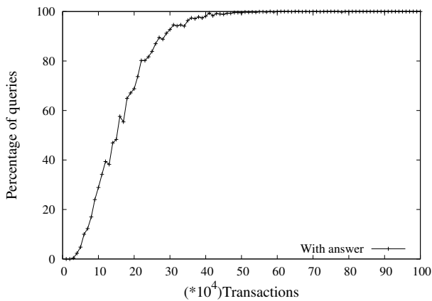
FIGURE 7. Hit ratio of the Trusted Ring
