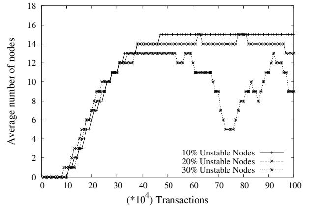
FIGURE 6. Size of the trustset on common nodes with respect to the churn ratio
