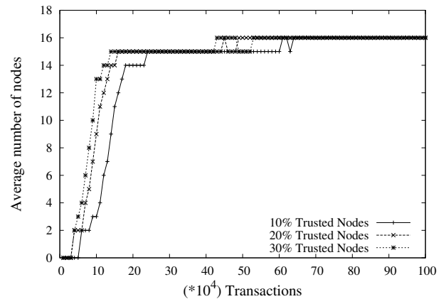
FIGURE 4. Size of the trustset on trusted nodes
