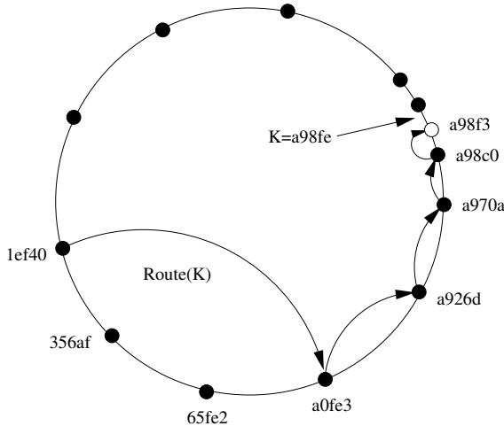
FIGURE 1. Routing example in Pastry: Route of key a98fe arrive to the node with the closest nodeID a98f3 .
