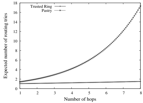
FIGURE 3. Number of expected routing attempts with respect to the number of hops
