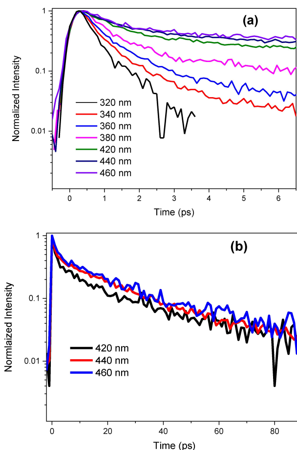
Figure 3. Total fluorescence decays over a time window of 10 ps (a) and 100 ps (b) on a semi-logarithmic scale, obtained from a solution of \epsilon dG in PBS pH 7.4 at different emission wavelengths after excitation at \lambda_{\text{exc}}=267\text{ nm} .
