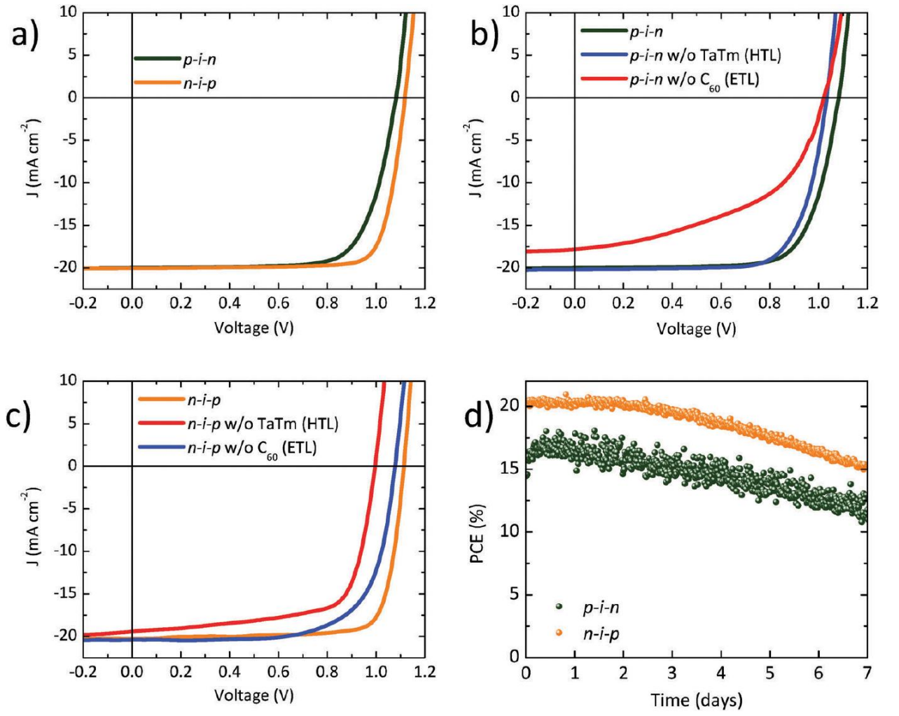
Fig. 4 (a) J - V curves for the n-i-p and p-i-n solar cells under 100 mW cm -2 illumination. (b) J - V curves under 100 mW cm -2 illumination for the p-i-n devices without one of the undoped charge transport layers. (c) J - V curves under 100 mW cm -2 illumination for n-i-p devices without one of the undoped charge transport layers. (d) Stability under approximated 100 mW cm -2 illumination.
