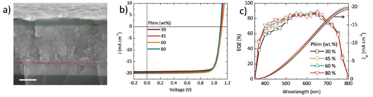
Fig. 3 (a) Cross-sectional SEM image of a completed n-i-p solar cell (scale bar 200 nm). (b) J–V curves under 100 \text{ mW cm}^{-2} illumination and (c) EQE spectra (the integrated photocurrent with the AM1.5G solar spectrum is shown on the right axis) as a function of PhIm concentration.
