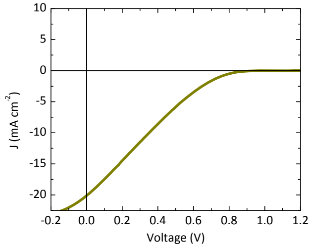
Fig. S3 J-V scan for a p-i-n device with the structure ITO/TaTm (40 nm)/MAPbI 3 (500 nm)/ C 60 (40 nm)/Ag.
