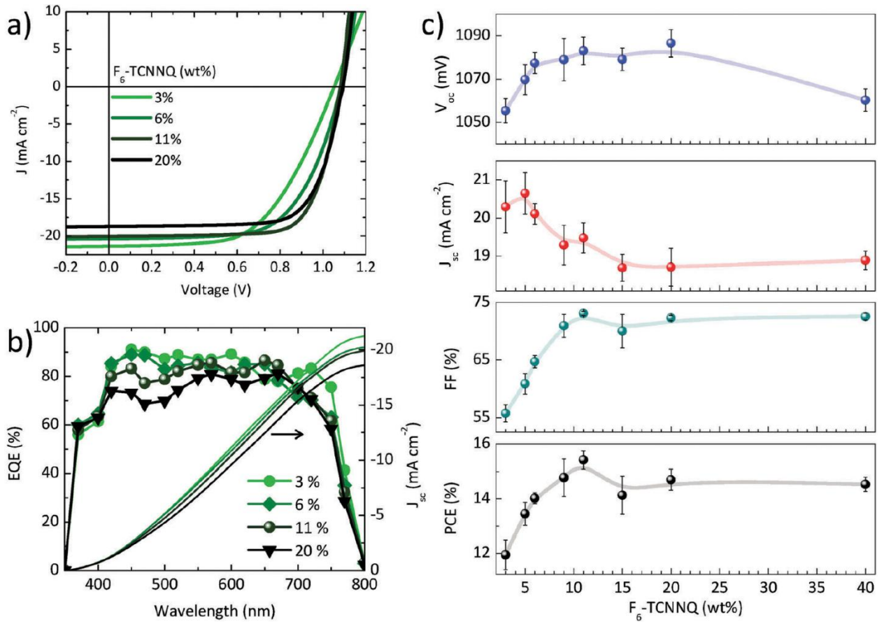
Fig. 2 (a) J - V curves under 100 mW cm 2 illumination and (b) external quantum efficiency (EQE) as a function of F 6 -TCNNQ concentration for the p-i-n solar cells (the integrated photocurrent with the AM1.5G solar spectrum is shown on the right axis). (c) Evolution of the key parameters deduced from the J - V curves, V_{oc} , J_{sc} , FF and PCE, as a function of F 6 -TCNNQ concentration.
