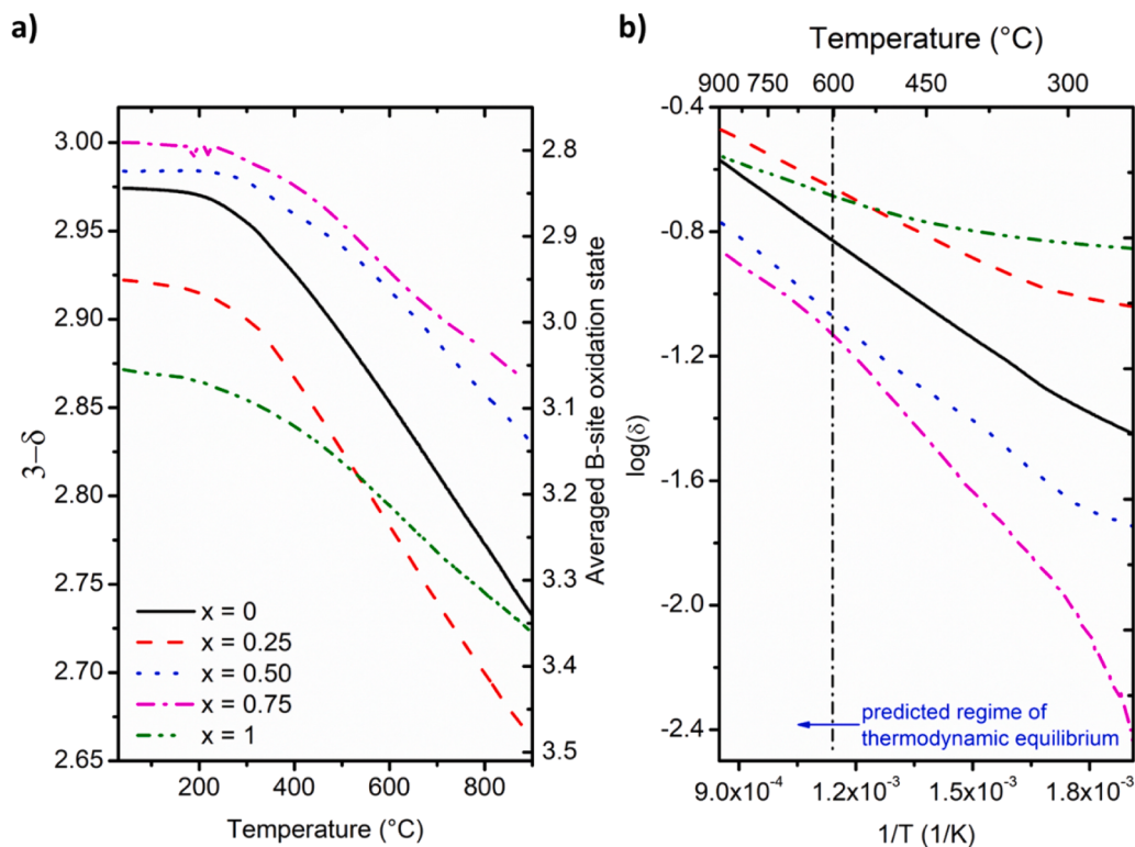
Fig. 2. Oxygen nonstoichiometry ( 3-\delta ) and averaged B-site oxidation state in synthetic air as a function of temperature upon cooling (a) and van 't Hoff plots of the concentration of oxygen vacancies (b).
