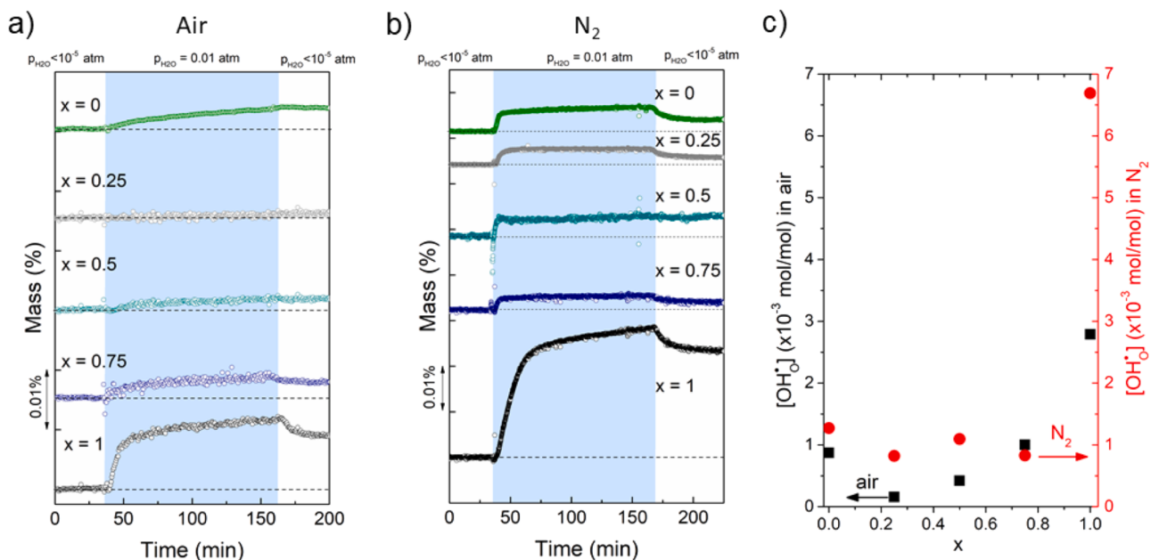
Fig. 7. Water uptake at 300 °C of \text{La}_{0.5}\text{Ba}_{0.5}\text{Co}_{1-x}\text{Fe}_x\text{O}_{3-\delta} measured in air (a) and nitrogen (b) as well as estimated concentration of protonic defects (c).
