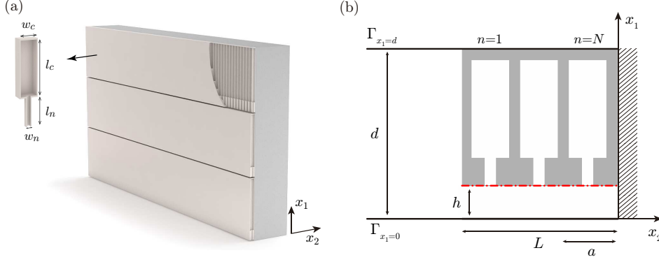
FIG. 1. (a) Conceptual view of the thin panel placed on a rigid wall with one layer of square cross-section Helmholtz resonators, N = 1 . (b) Scheme of the unit cell of the panel composed of a set of N Helmholtz resonators. Symmetry boundary conditions are applied at boundaries \Gamma_{x_1=d} and \Gamma_{x_1=0} .
