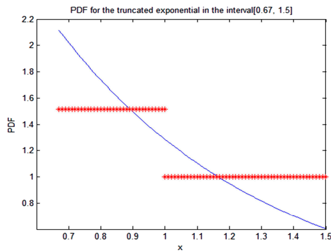
Figure 10. Probability distribution obtained using the MEP for the parameter f_K in the interval [0.67, 1.5], blue decreasing line. The red line is the histogram from reference [30].
