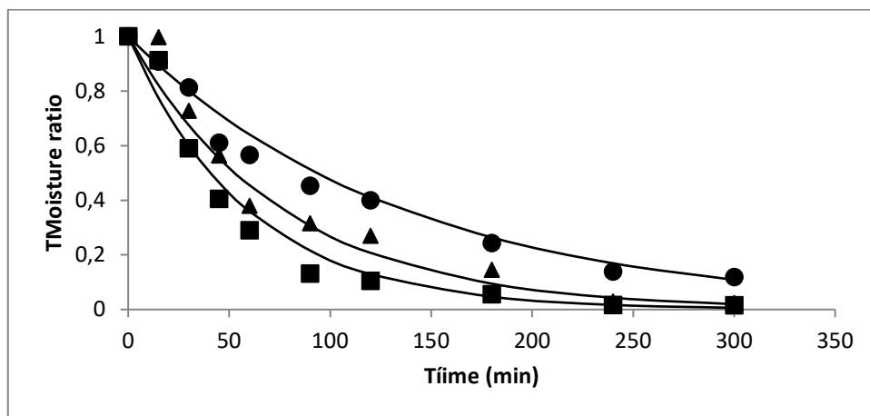
Fig. 1 Drying kinetics of C. pubescens samples of 1 cm thickness ( \blacktriangle=70^{\circ}\text{C} , \bullet=60^{\circ}\text{C} , \blacksquare=50^{\circ}\text{C} )
