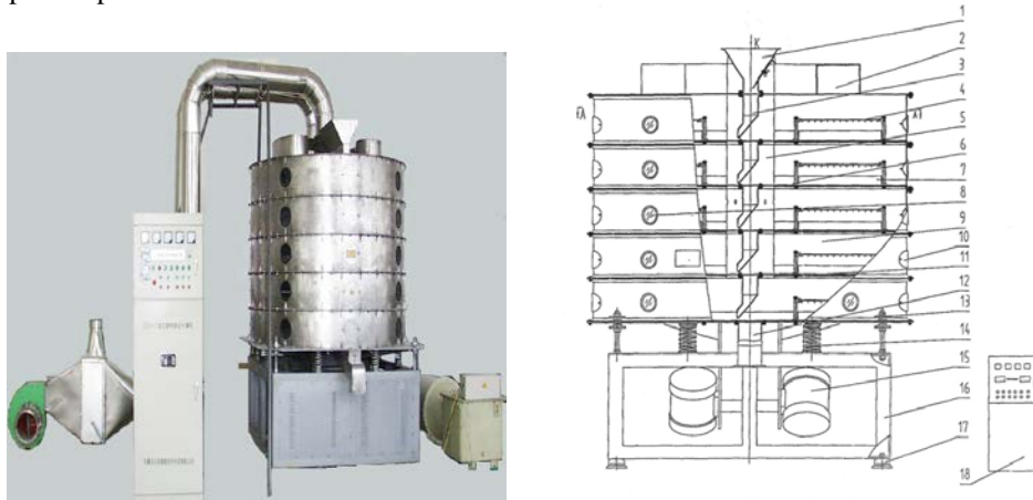
Fig. 2 The picture and schematics of the EHD dryer model GTJ-1.7. [38]
