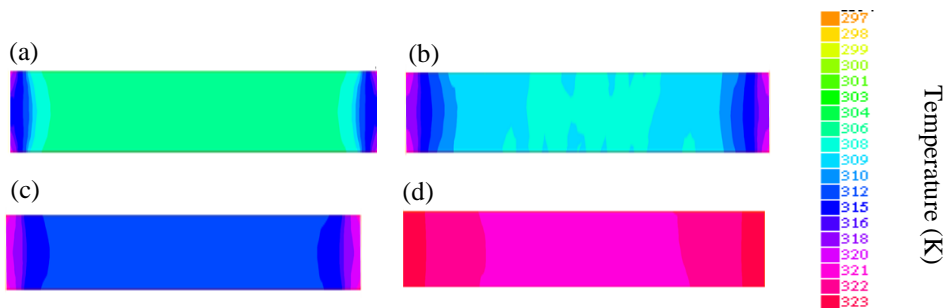
Fig 4. Temperature distribution inside the slice during drying simulation by the finite elements method. (a) 3000 s. (b) 6000 s. (c) 12000 s. (d) 15000 s.
