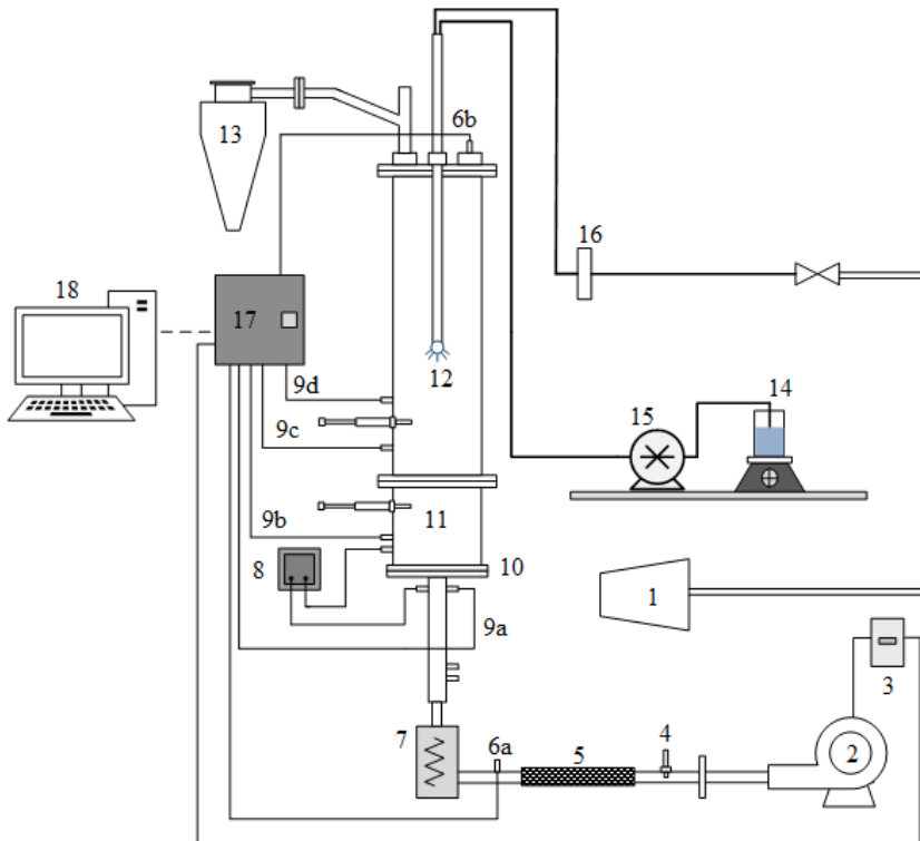
Fig 1. Experimental System
