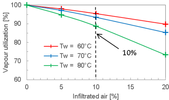
Fig. 6 Potential of waste vapour heat recovery and temperature level of this heat
