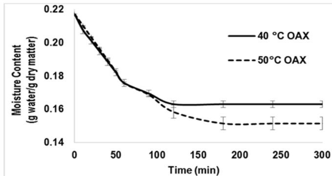
Fig. 4 Drying kinetics of mesquite pods stage 3 at 40 °C and 50 °C (Oaxaca).
