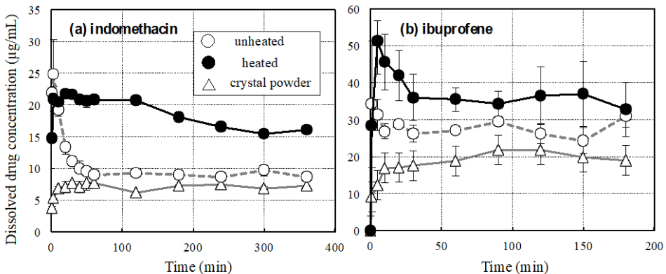
Fig. 2. Dissolution profiles of (a) indomethacin and (b) ibuprofene in water from unheated and heated surfactant-free solid dispersion as well as crystalline powders of model drugs. \alpha -Maltose was used as sugar, and the drug content in the solid dispersion sample was 1% w/w. The amounts of model drug added to the water were 50 \mu\text{g/mL} for (a) indomethacin and 500 \mu\text{g/mL} for (b) ibuprofene. The heat-treatment was conducted at 120°C for 60 min.
