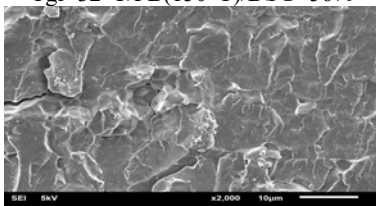
T_{gi}=32^{\circ}\text{C}/\text{FB}(170^{\circ}\text{C})\text{MW}(2.4\text{kW})/\text{DSG}=70\%
