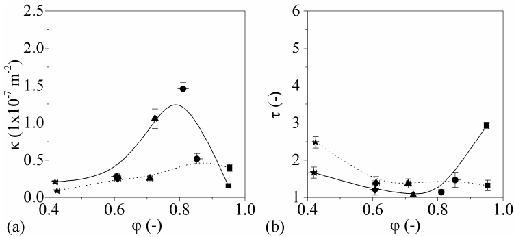
Fig. 3 Packed-bed parameters as a function of \varphi for alumina (■), soy (●), lentil (▲), barley (◆) and oats (★); \kappa (a) and \tau (b). Legend: moistures contents of 24% (—) and X_{eq} (.....).
