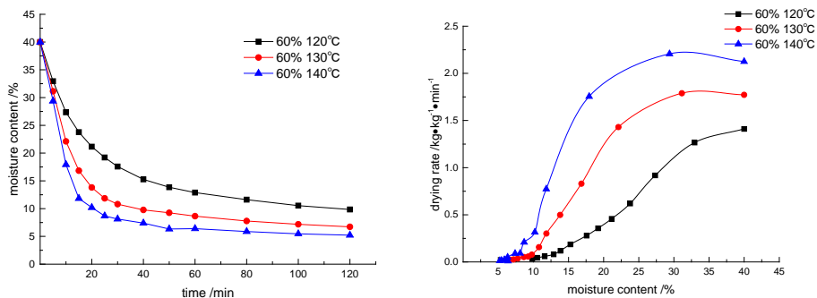
(a) Drying curves (60%)
