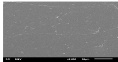
T_{gi}=55^{\circ}\text{C}/\text{FB}(170^{\circ}\text{C})\text{MW}(2.4\text{kW})/\text{DSG}=96\%
