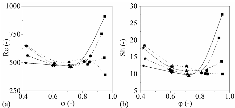
Fig. 4. Estimated values of Re (a) and Sh (b) as a function of \phi for alumina (■), soy (●), lentil (▲), barley (◆) and oats (★) at 0.58 \text{ m}\cdot\text{s}^{-1} . Legend: moisture of 24% (—), 16% (---), 9% (-·-·-) and X_{eq} (·····).
