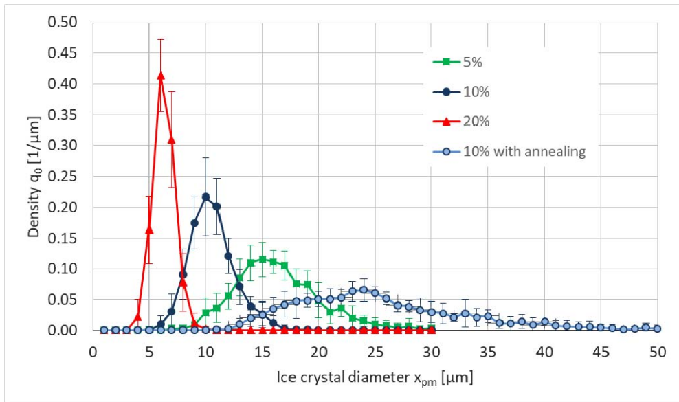
Fig. 3. Ice crystal diameter for frozen maltodextrin solutions at -50°C for different solid contents. Freezing was carried out with a cooling rate of 20 K/min. For the 10% solution, the ice crystal size distribution for annealing treatment II (-5°C/180min) is also shown
