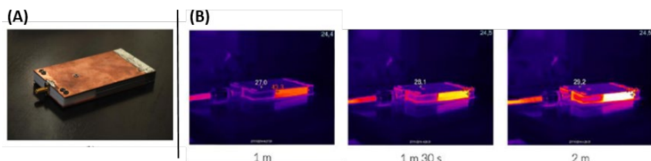
Fig. 1. Picture of stripline radiators (A) and, (B) Thermographies of a heating cycle, applying 30 W microwave power at 2.45 GHz per cell, on the right [24] .
