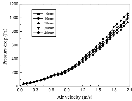
Fig. 4 Variations in pressure drop at different distance between distributors
