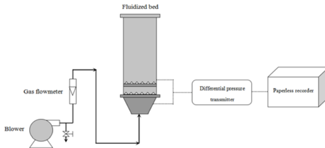
Fig. 1 Experimental flow chart.
