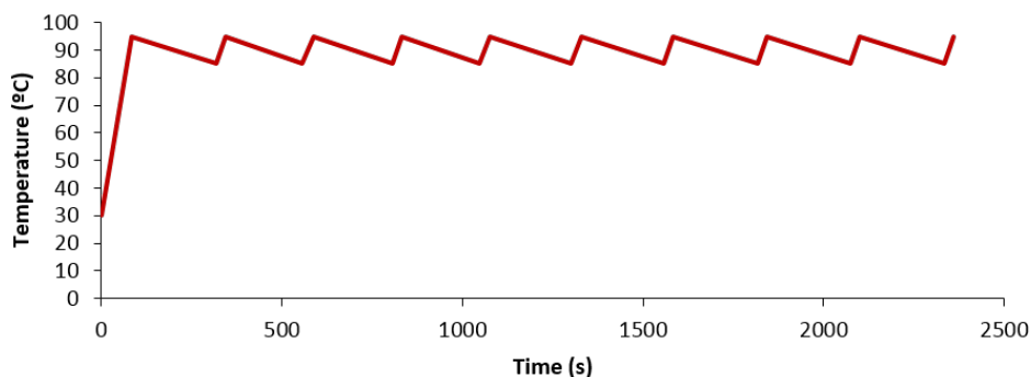
Fig. 2. Temperature variation of the surface of a 300 W prototype [26] .
