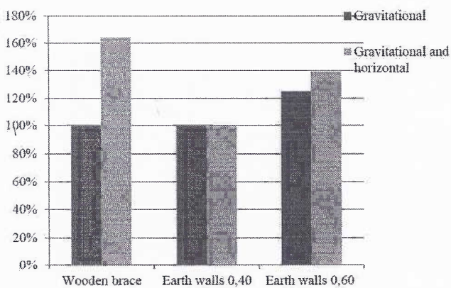
Fig. 10 Coefficient breaking reference
