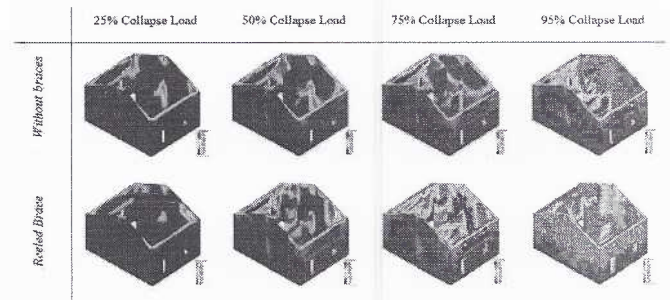
Fig. 8 Evolution of damages according to increasing loads
