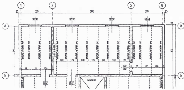
Fig. 4 Nonlinear static method, bearing gravitational and horizontal loads until collapse. Axis Sx
