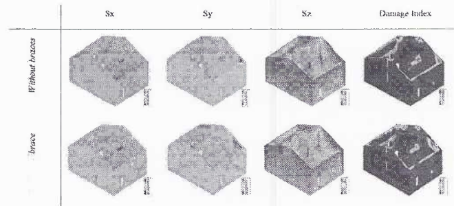
Fig. 2 Static lineal method using gravitational and wind pressure
