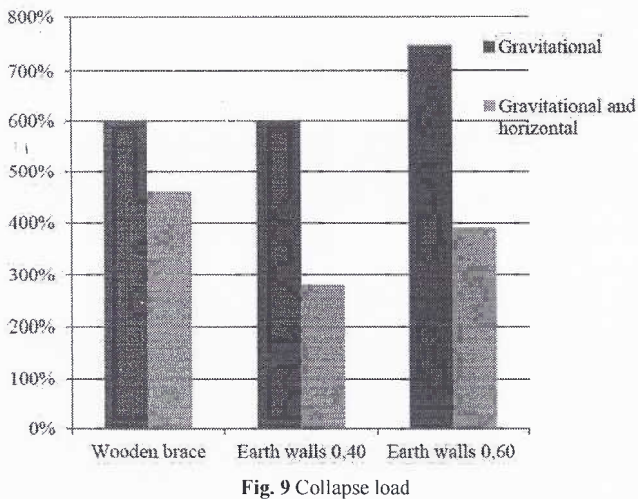
Fig. 9 Collapse load
