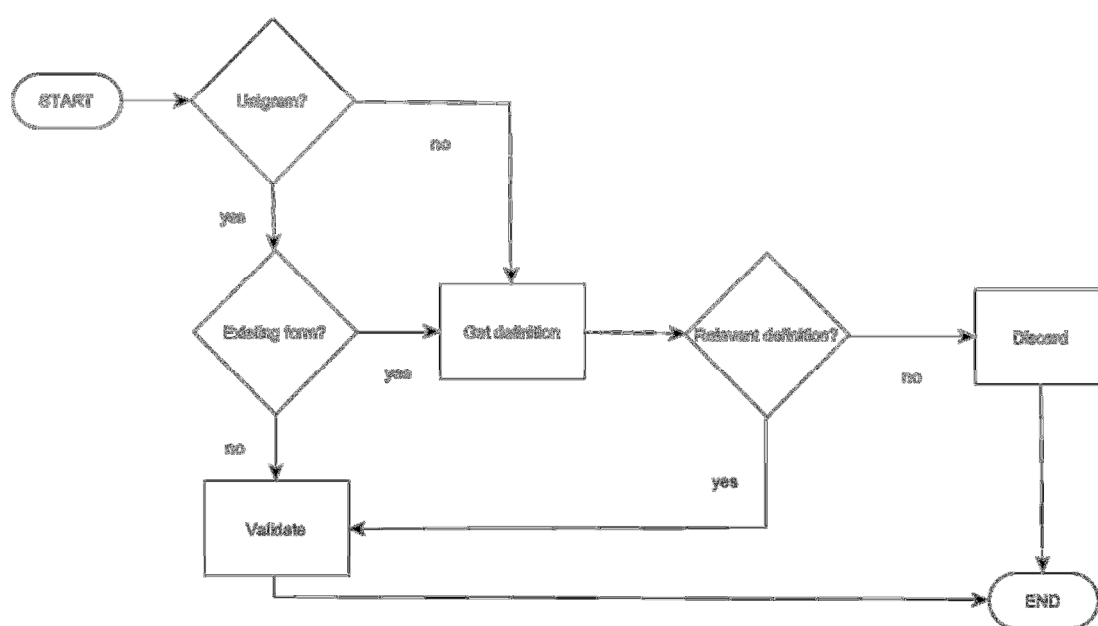
Figure 5. Flowchart for term validation.
