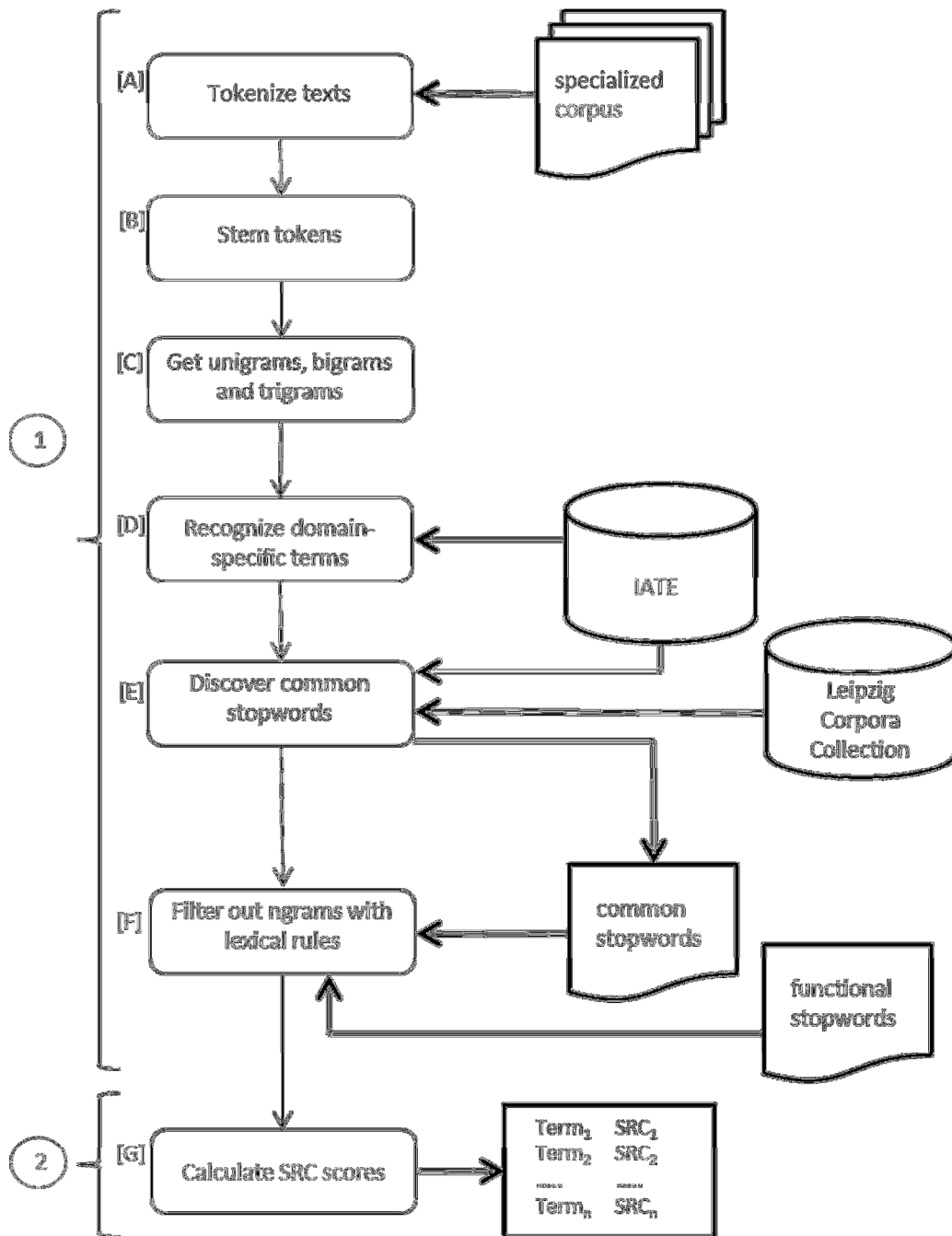
Figure 1. DEXTER Web service: workflow of term extraction.
