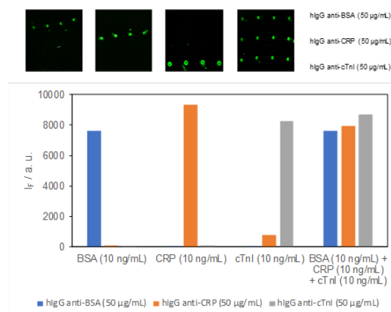
Fig. 6 Multiplexing assay in the microarray format for protein/antibody systems: BSA/hlgG \alpha BSA, CRP/hlgG \alpha CRP and cTnI/hlgG \alpha cTnI. Incubating with (A) BSA* (10 ng/mL); (B) CRP* (10 ng/mL); (C) cTnI (10 ng/mL); (D) mixture of BSA* (10 ng/mL), CRP* (10 ng/mL) and cTnI (10 ng/mL).
