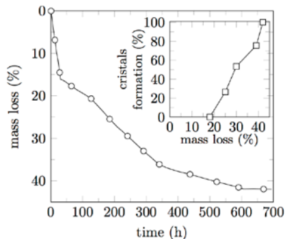
Fig. 3 Mass loss and crystals formation during static syntheses
